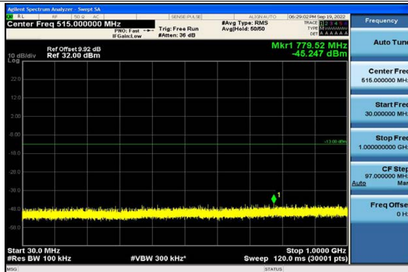
Band4-3MHz-QPSK-20175-1RB#0-30~1000MHz
