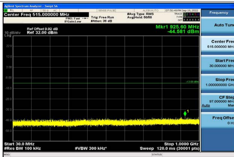
Band4-20MHz-16QAM-20050-1RB#0-30~1000MHz
