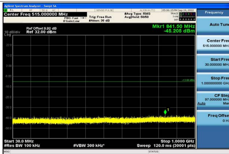
Band2-15MHz-QPSK-18675-1RB#0-30~1000MHz
