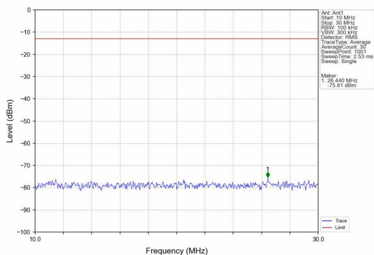
Band12 3MHz 16QAM MCH 707.5MHz RB 1 0 NTV
