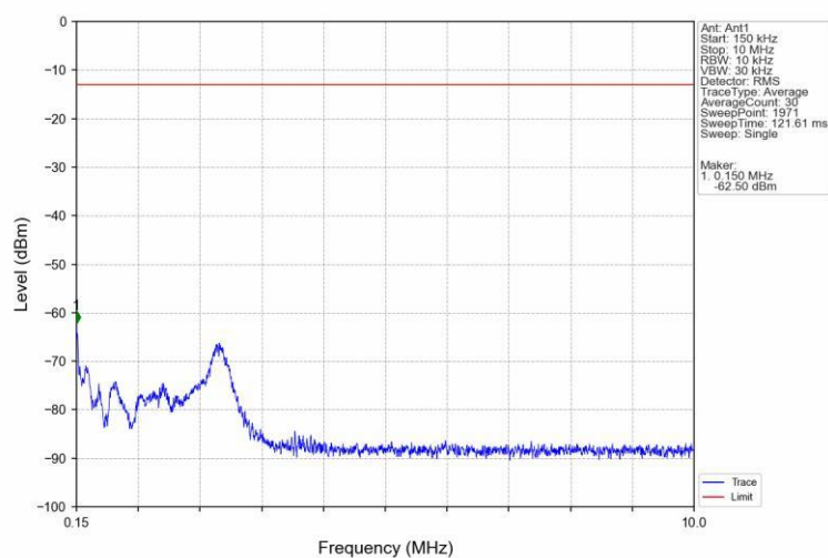
Band12 3MHz QPSK HCH 714.5MHz RB 1 0 NTN
