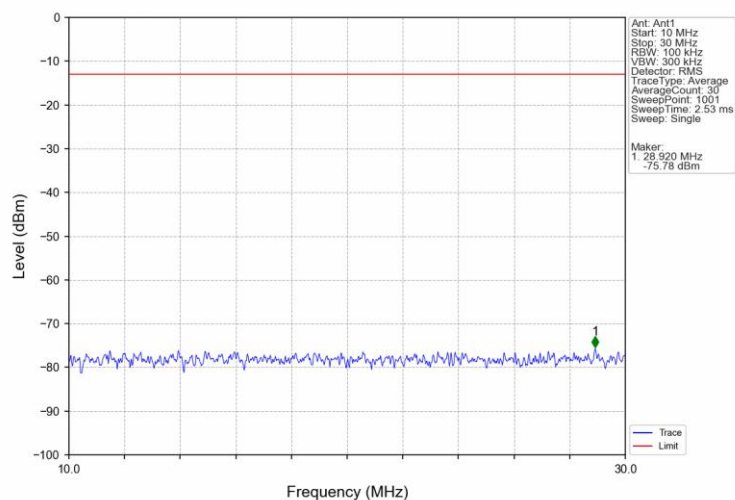
Band12 10MHz QPSK HCH 711MHz RB 1 0 NTNV
