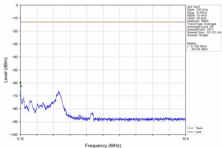
Band12 10MHz QPSK LCH 704MHz RB 1 0 NTN
