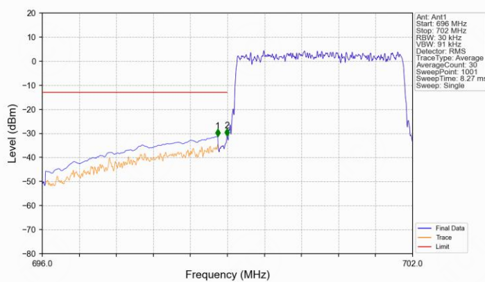
Band12 3MHz 16QAM LCH 700.5MHz RB 15 0 NTV
