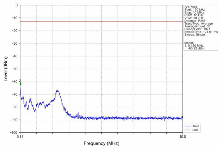
Band12 3MHz 16QAM MCH 707.5MHz RB 1 0 NTV
