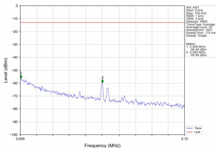
Band12 3MHz QPSK MCH 707.5MHz RB 1 0 NTNV
