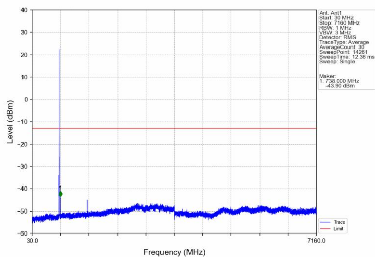
Band12 3MHz 16QAM MCH 707.5MHz RB 1 0 NTV
