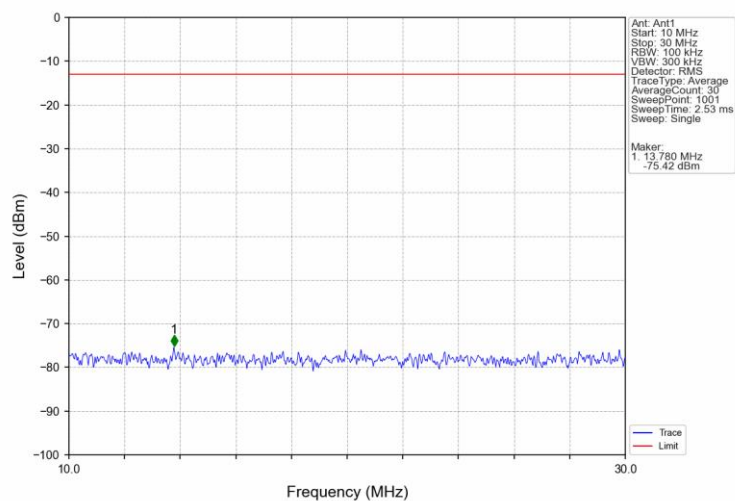
Band12 10MHz QPSK LCH 704MHz RB 1 0 NTN
