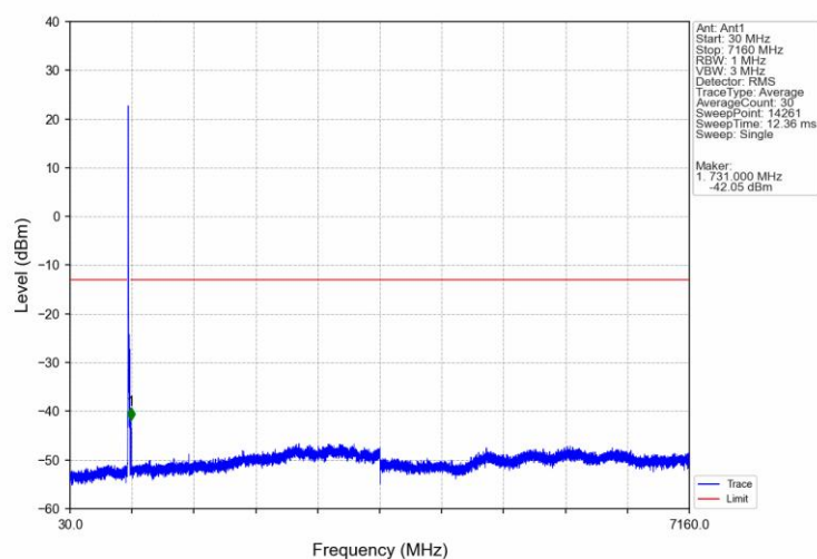
Band12 10MHz QPSK LCH 704MHz RB 50 0 NTN
