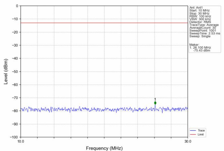
Band12_3MHz_16QAM_LCH_700.5MHz_RB_1_0_NTNV
