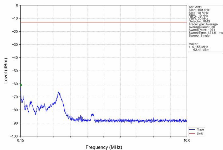
Band12 10MHz QPSK HCH 711MHz RB 1 0 NTNV
