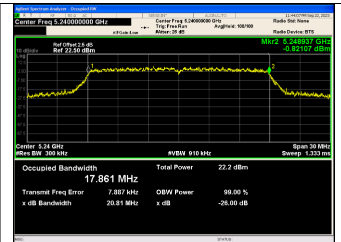
IEEE 802.11ac Channel 48 20MHz Antenna 1
