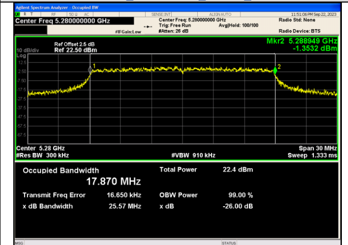
IEEE 802.11ac Channel 56 20MHz Antenna 1
