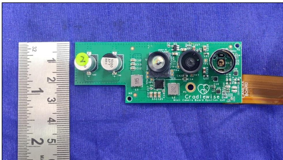
Photo 18: Camera board
