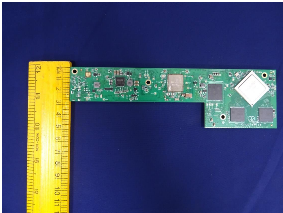
Photo 24: Compute board with dimensioned view
