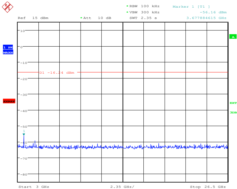
(Plot 4.6.1 C2: Channel 11: 2462MHz @ 802.11b)
