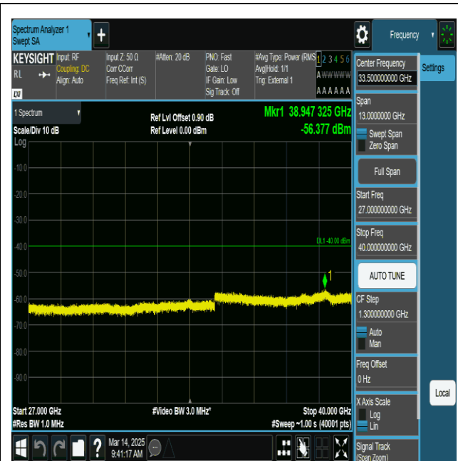
Band48-20MHz-QPSK-55990-1RB#0-27000~40000-PASS
