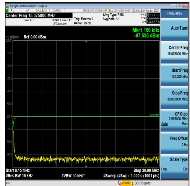
Band48-20MHz-QPSK-56640-1RB#0-0.15~30-PASS
