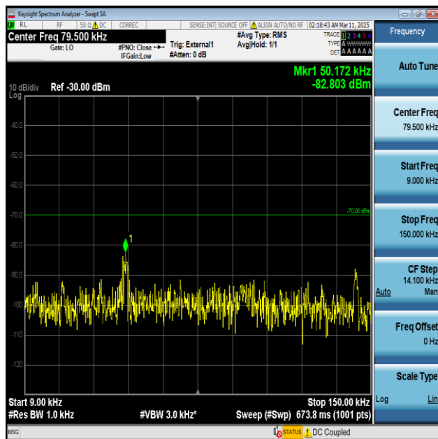
Band48-20MHz-QPSK-56640-1RB#0-0.009~0.15-PASS
