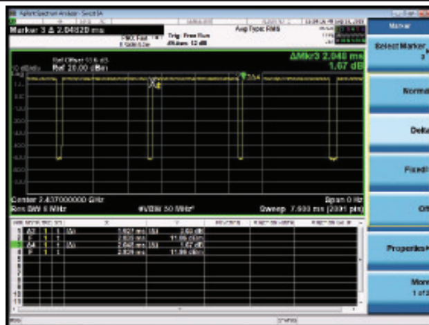
802.11ac-VHT20 (T = 1.93ms)
