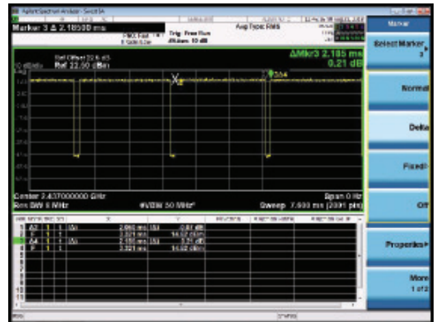
802.11n-HT40 (T = 938.60us)
