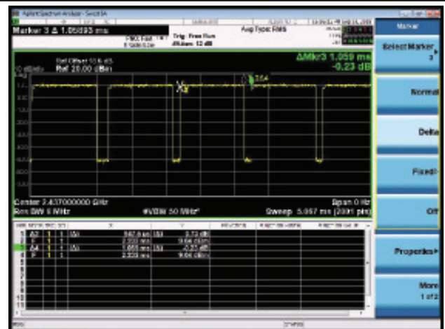
802.11ac-VHT40 (T = 947.50us)
