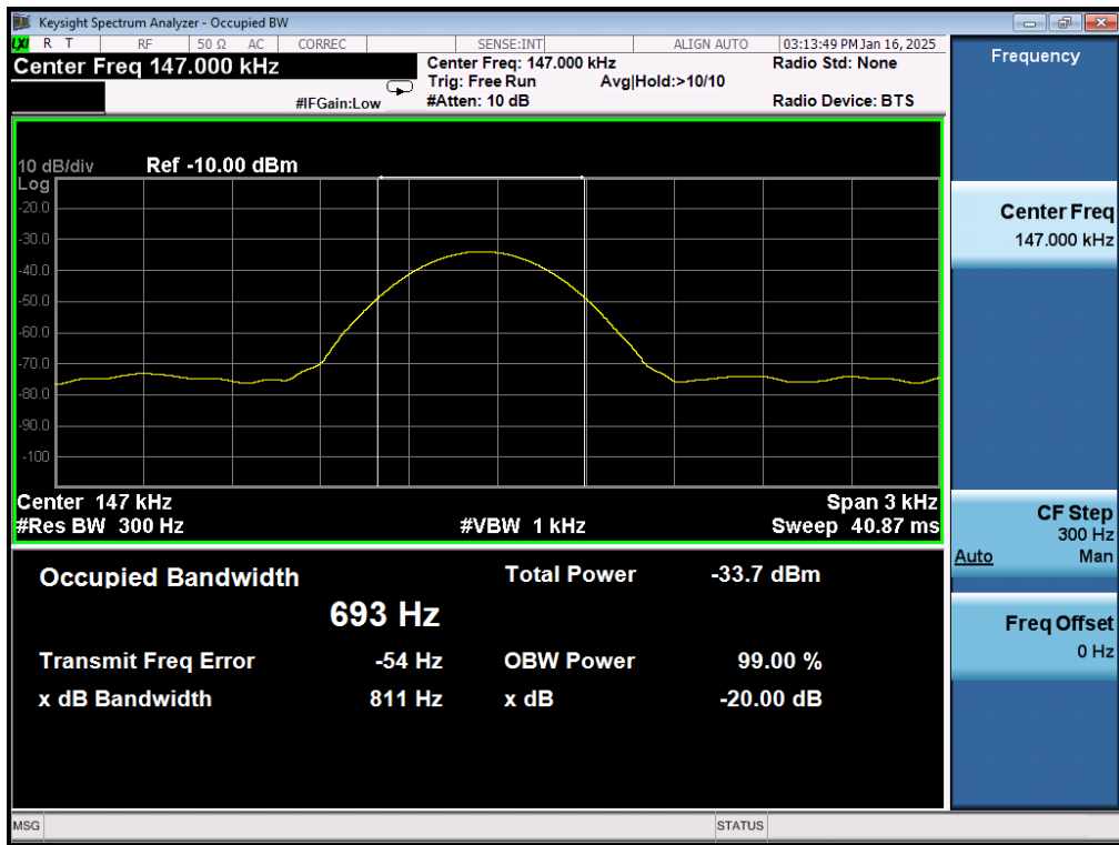
Test_Graph_ASK_Coil_147.0kHz_-20dB Bandwidth
