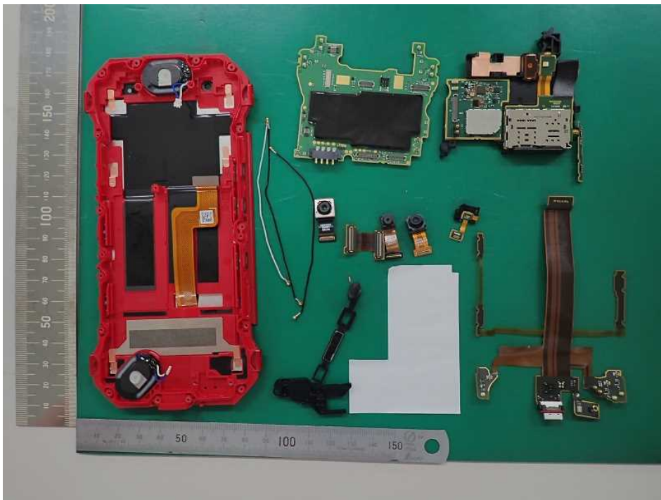
Rear cover open 5
