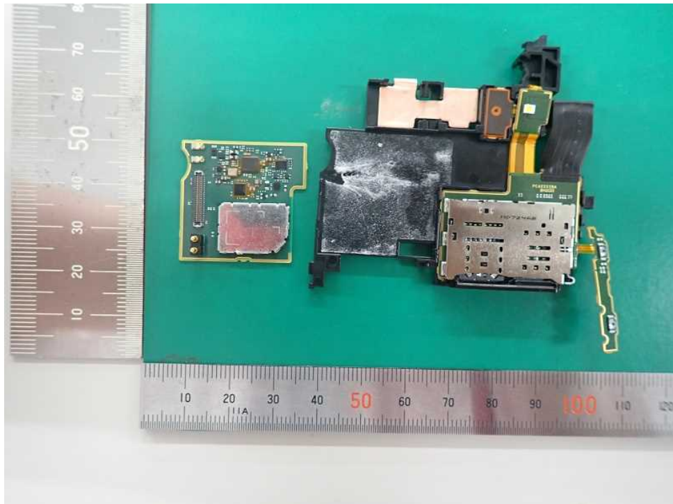
Sub PCB 1
