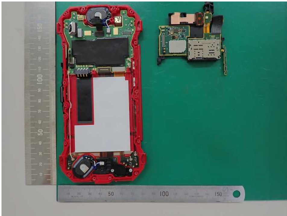
Rear cover open 3
