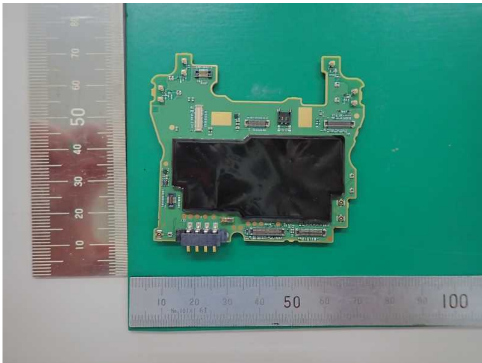
Main PCB rear 1
