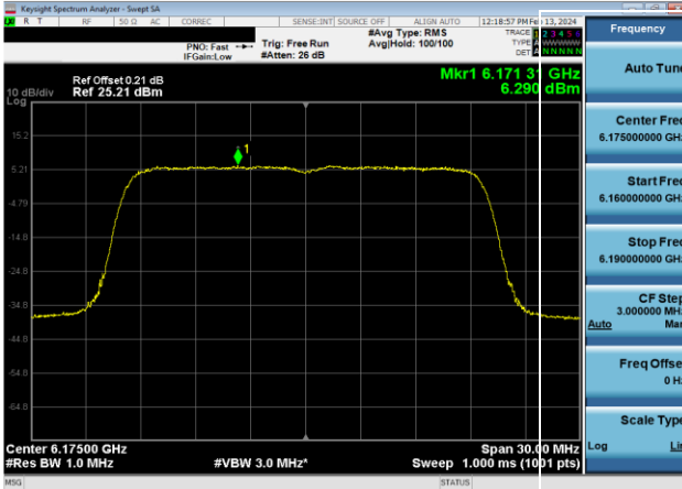
Plot 7-565. Power Spectral Density Plot CDD Primary Antenna WF8 Standard Power (20MHz 802.11ax (UNII Band 5) - Ch. 45, MCS4)
