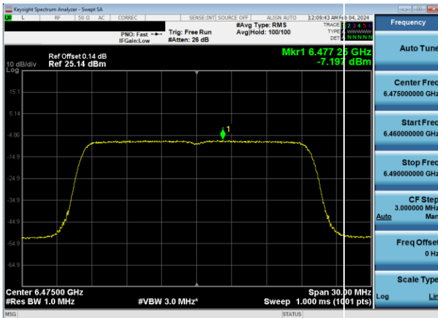
Plot 7-604. Power Spectral Density Plot SDM Diversity Antenna WF8 LPI (20MHz 802.11ax (UNII Band 6) – Ch. 105, MCS2)
