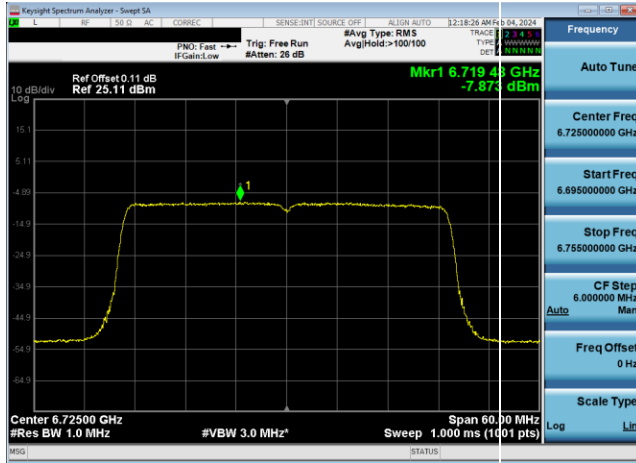
Plot 7-614. Power Spectral Density Plot SDM Diversity Antenna WF8 LPI (40MHz 802.11ax (UNII Band 7) – Ch. 155, MCS2)
