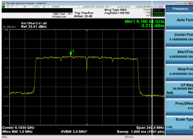
Plot 7-587. Power Spectral Density Plot CDD Primary Antenna WF8 Standard Power (160MHz 802.11ax (UNII Band 5) – Ch. 47, MCS11)
