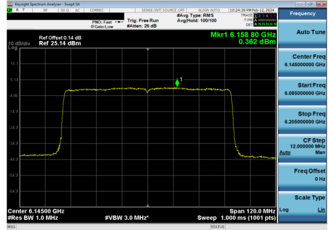
Plot 7-552. Power Spectral Density Plot CDD Primary Antenna WF8 Standard Power (80MHz 802.11ax (UNII Band 5) – Ch. 39, MCS2)
