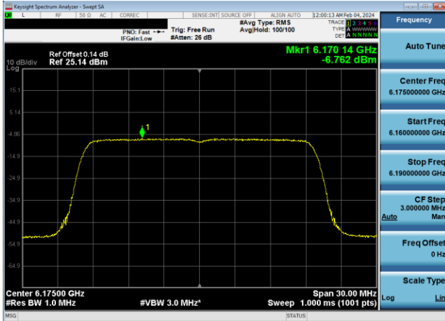
Plot 7-596. Power Spectral Density Plot SDM Diversity Antenna WF8 LPI (20MHz 802.11ax (UNII Band 5) – Ch. 45, MCS2)
