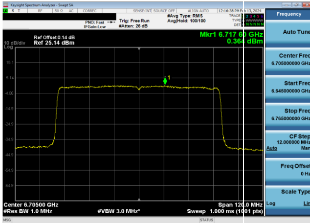
Plot 7-561. Power Spectral Density Plot CDD Primary Antenna WF8 Standard Power (80MHz 802.11ax (UNII Band 7) - Ch. 151, MCS2)
