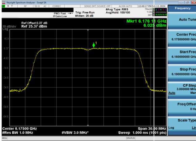
Plot 7-580. Power Spectral Density Plot CDD Primary Antenna WF5B Standard Power (20MHz 802.11ax (UNII Band 5) – Ch. 45, MCS11)
