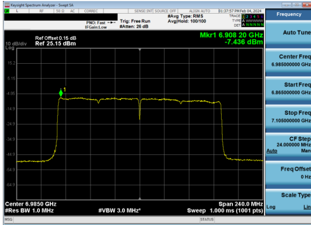
Plot 7-627. Power Spectral Density Plot SDM Diversity Antenna WF7 LPI (160MHz 802.11ax (UNII Band 8) – Ch. 207, MCS2)
