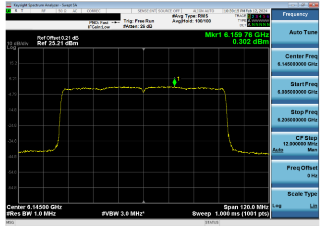
Plot 7-568. Power Spectral Density Plot CDD Primary Antenna WF5B Standard Power (80MHz 802.11ax (UNII Band 5) - Ch. 39, MCS4)
