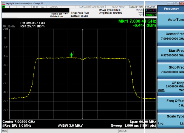
Plot 7-622. Power Spectral Density Plot SDM Diversity Antenna WF8 LPI (40MHz 802.11ax (UNII Band 8) – Ch. 211, MCS2)
