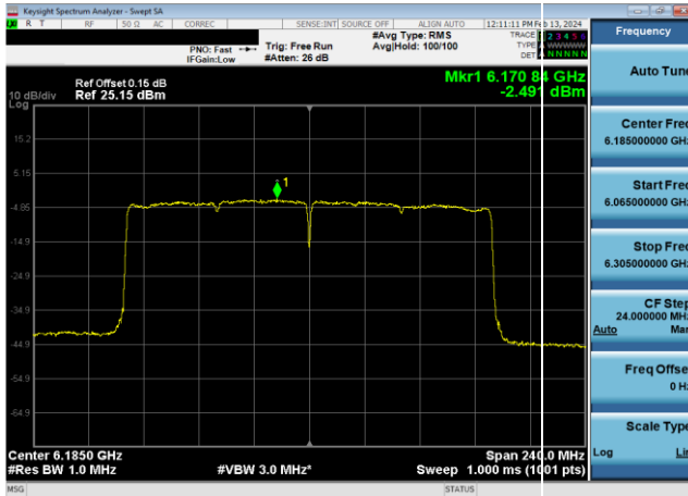
Plot 7-555. Power Spectral Density Plot CDD Primary Antenna WF8 Standard Power (160MHz 802.11ax (UNII Band 5) – Ch. 47, MCS2)
