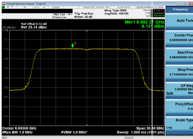
Plot 7-556. Power Spectral Density Plot CDD Primary Antenna WF5B Standard Power (20MHz 802.11ax (UNII Band 7) – Ch. 149, MCS2)
