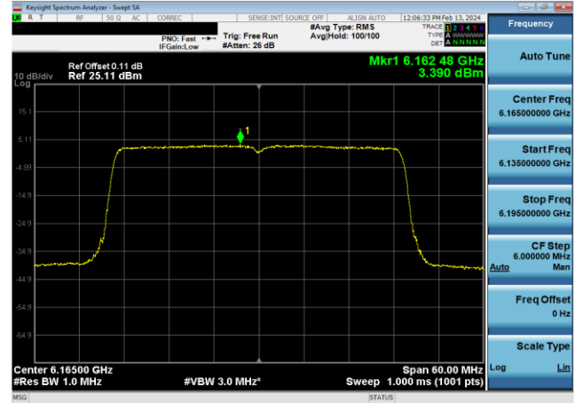
Plot 7-551. Power Spectral Density Plot CDD Primary Antenna WF8 Standard Power (40MHz 802.11ax (UNII Band 5) – Ch. 43, MCS2)
