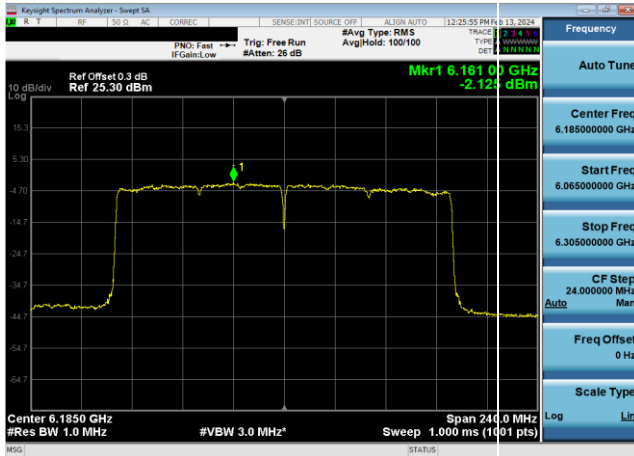
Plot 7-571. Power Spectral Density Plot CDD Primary Antenna WF8 Standard Power (160MHz 802.11ax (UNII Band 5) – Ch. 47, MCS4)
