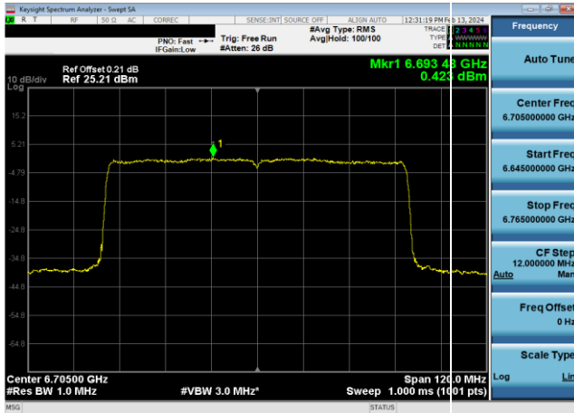
Plot 7-577. Power Spectral Density Plot CDD Primary Antenna WF8 Standard Power (80MHz 802.11ax (UNII Band 7) - Ch. 151, MCS4)
