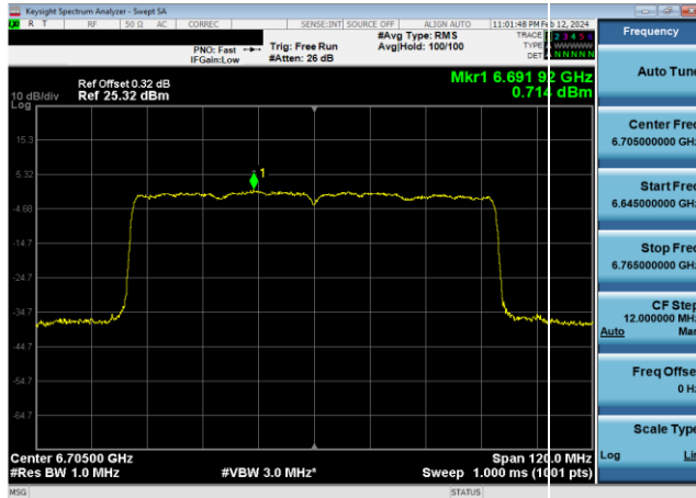
Plot 7-592. Power Spectral Density Plot CDD Primary Antenna WF5B Standard Power (80MHz 802.11ax (UNII Band 7) – Ch. 151, MCS11)
