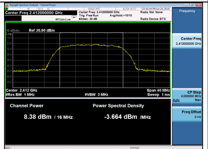
802.11g - PK Output power - Low CH 2412
