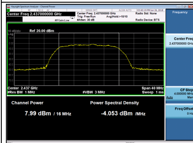
802.11g - PK Output power - Mid CH 2437
