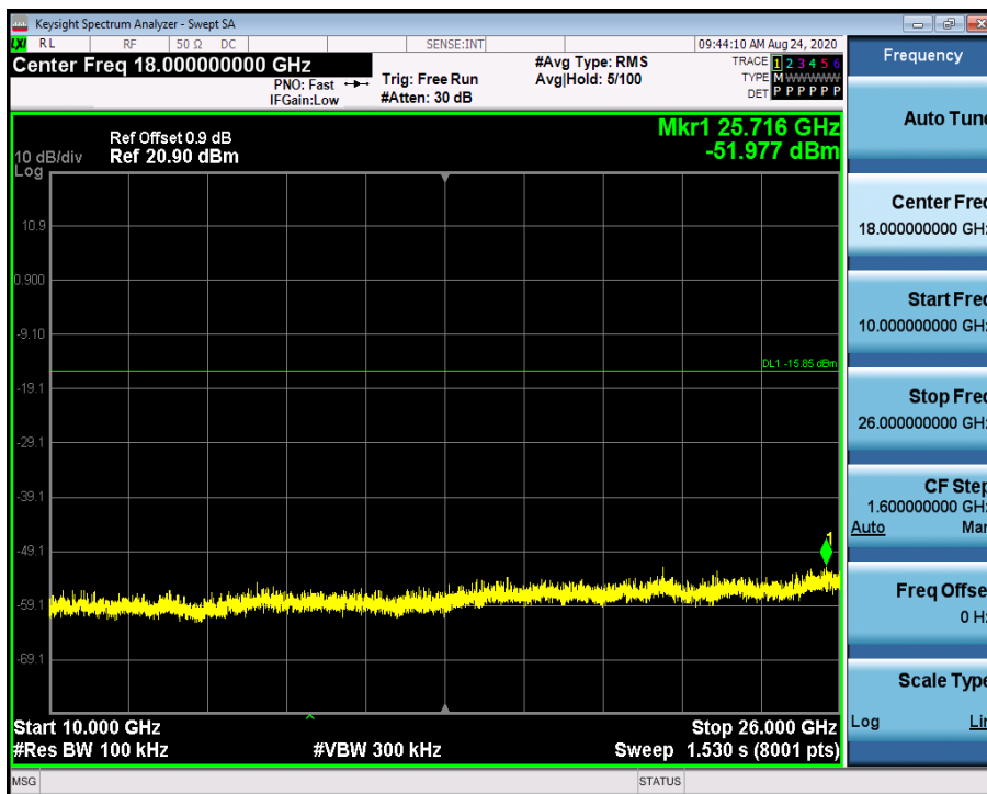
RF Conducted Spurious Emissions_2DH5_2480
