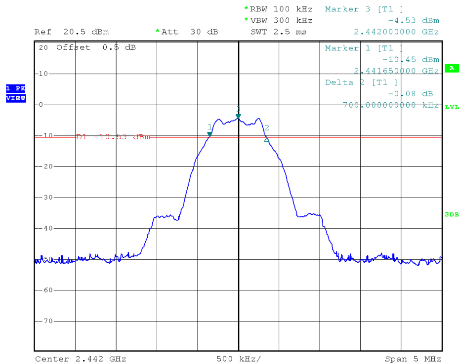
(Plot B1: Channel 20: 2442 MHz)
