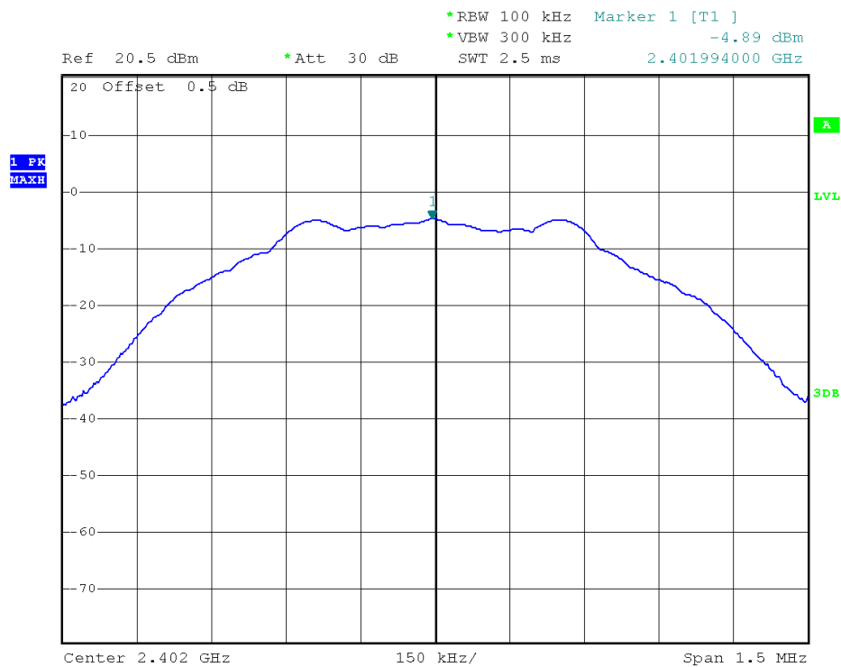
(Plot A: Channel = 0)
