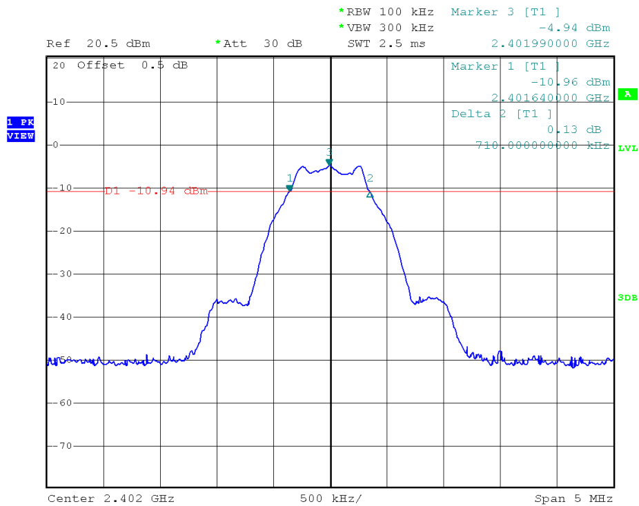
(Plot A1:Channel 0: 2402MHz)
