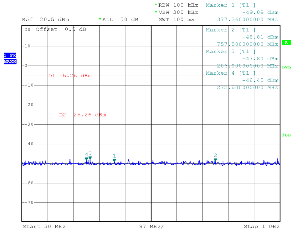
(Plot B.1: Channel = 20, 30MHz to 1GHz)
