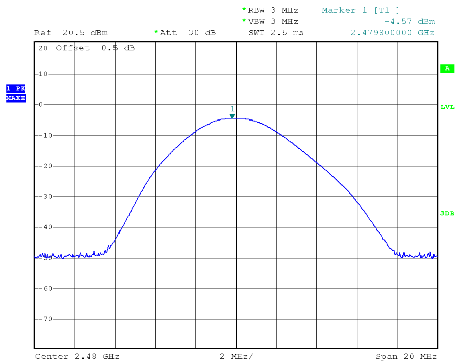
(Plot C: Channel 39: 2480MHz)
