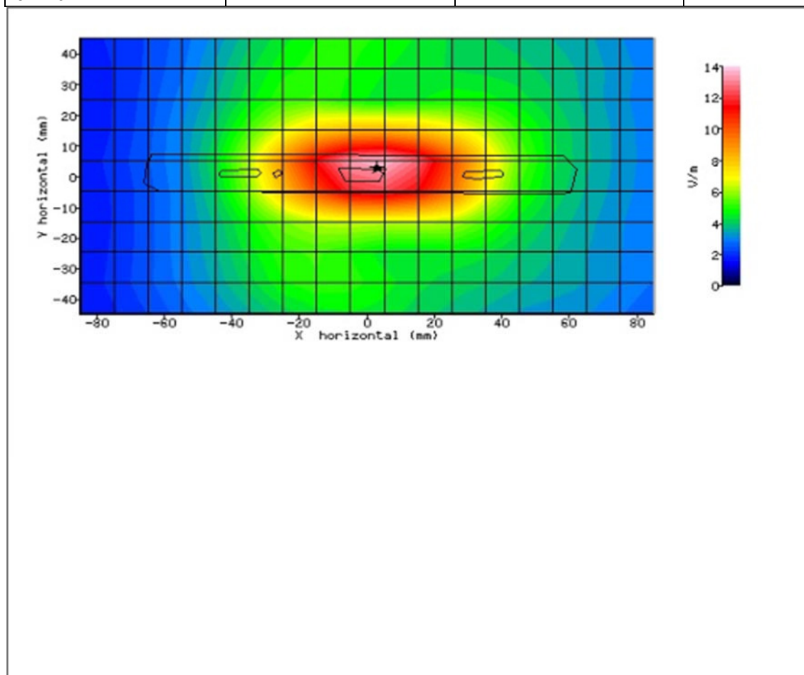
Figure 49: SAR Body Testing Results for the Sharp Smart phone at 782.0MHz.
