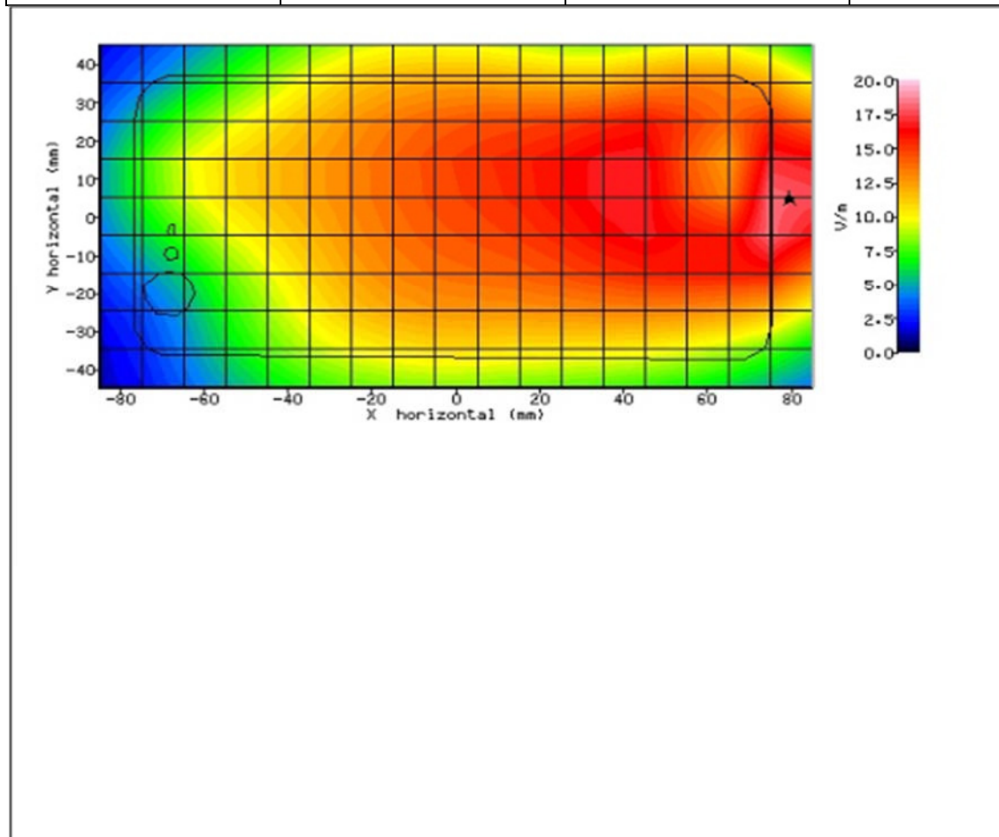
Figure 39: SAR Body Testing Results for the Sharp Smart phone at 829.0MHz.
