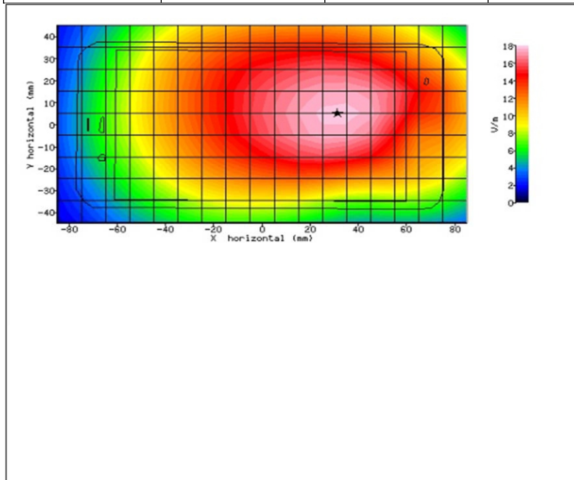
Figure 62: SAR Body Testing Results for the Sharp Smart phone at 710.0MHz.
