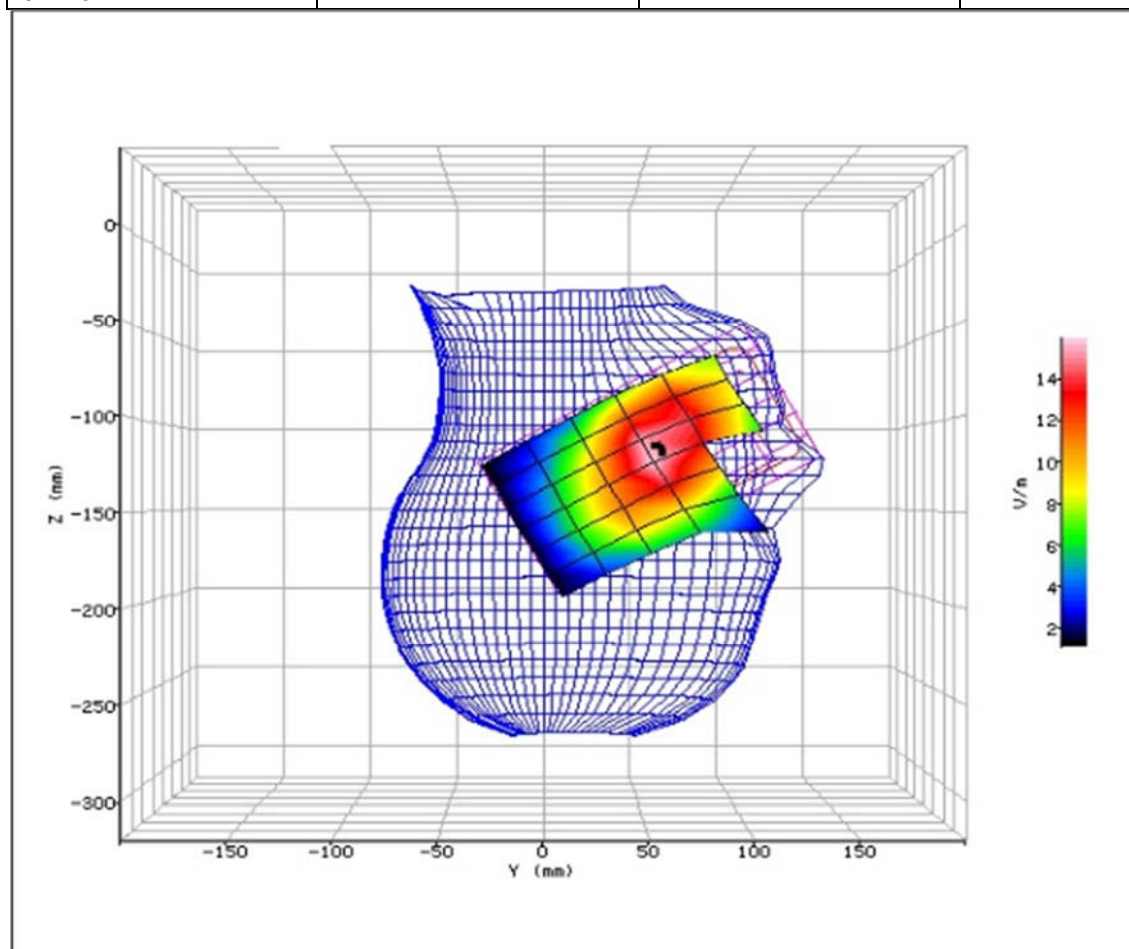
Figure 60: SAR Head Testing Results for the Sharp Smart phone at 710.0MHz.
