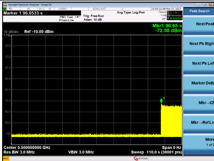
power-on cycle(5500MHz)
