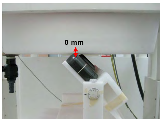
Fig.4 EUT Back side (WLAN Main) to flat phantom
