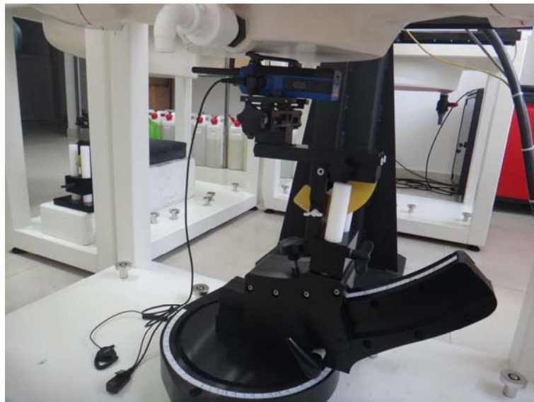
Body-worn, the front of the EUT towards ground with AA1
