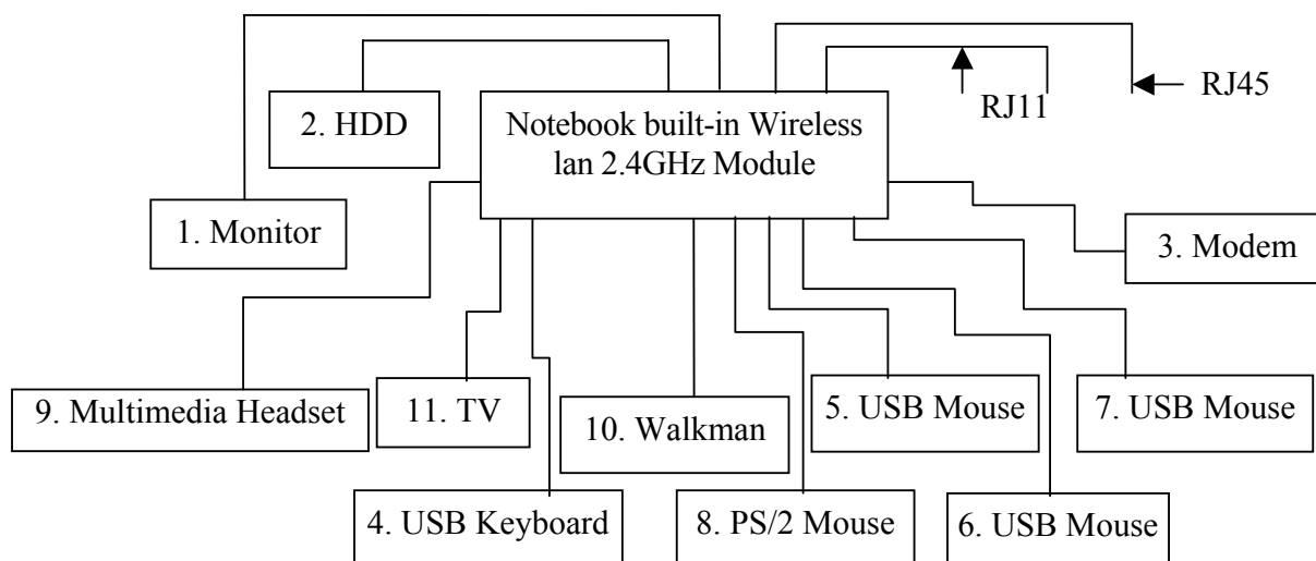
Fig. 2-1 Configuration of Tested System
