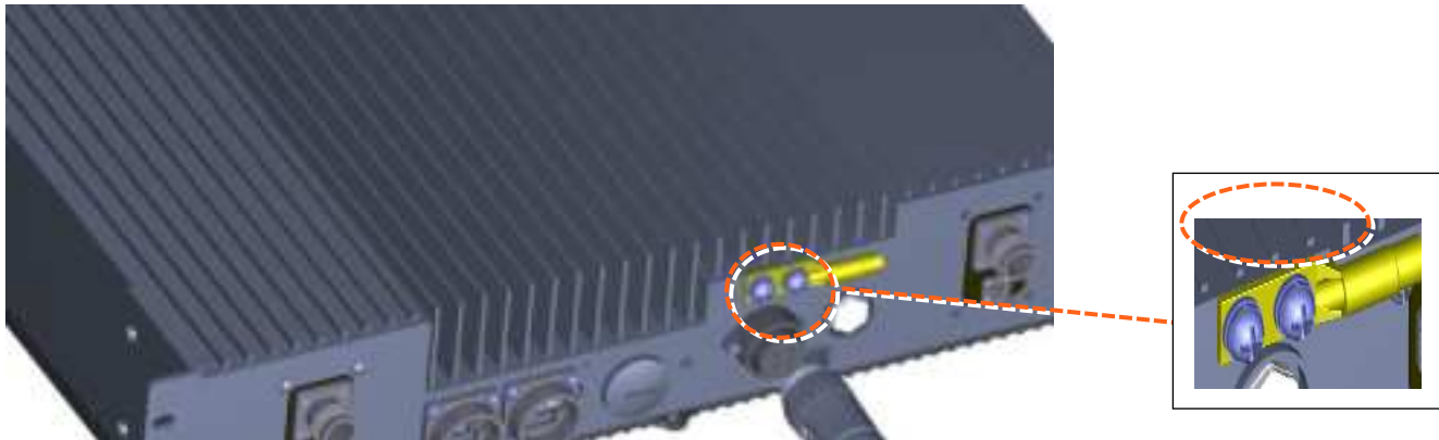
Figure 80. GND Connection
