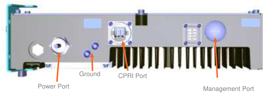
Figure 84. dHRU Front View
