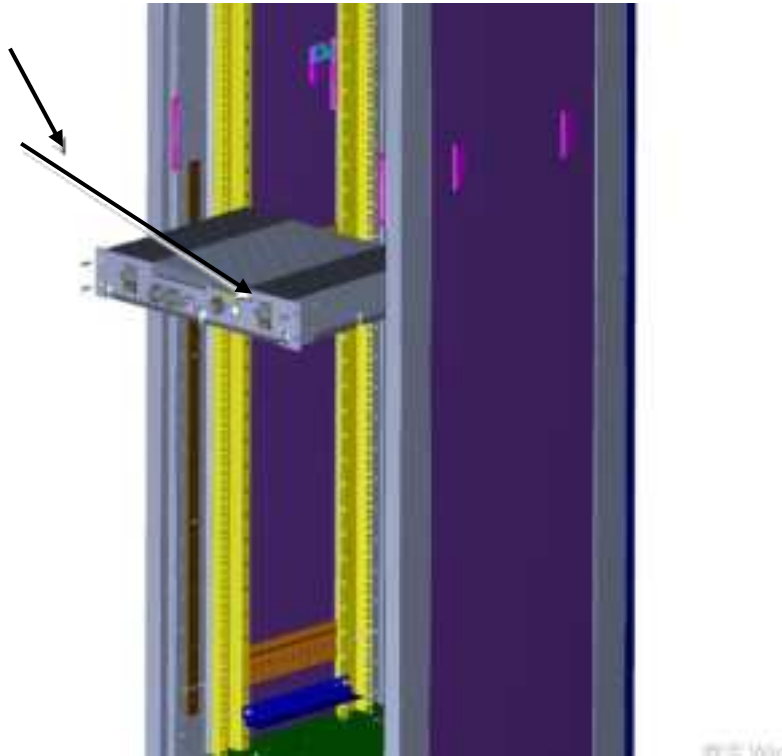
Figure 76. Rack Installation
