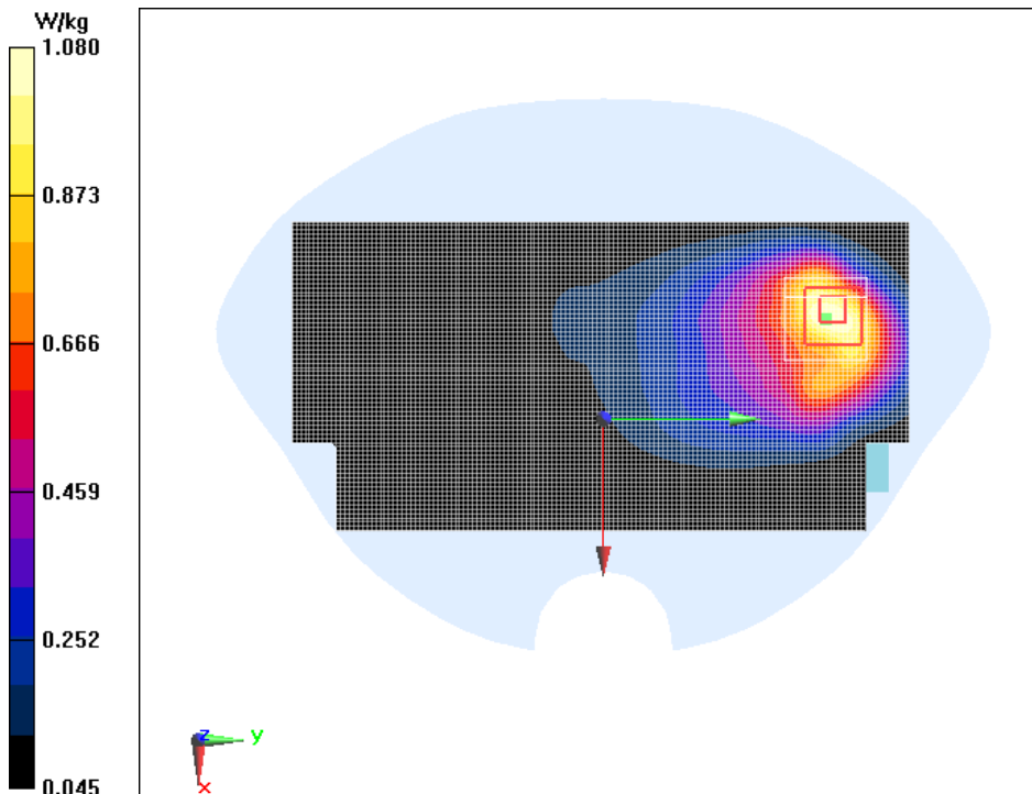
Fig.1 GSM850 Phantom 4TS Mode High 0mm
