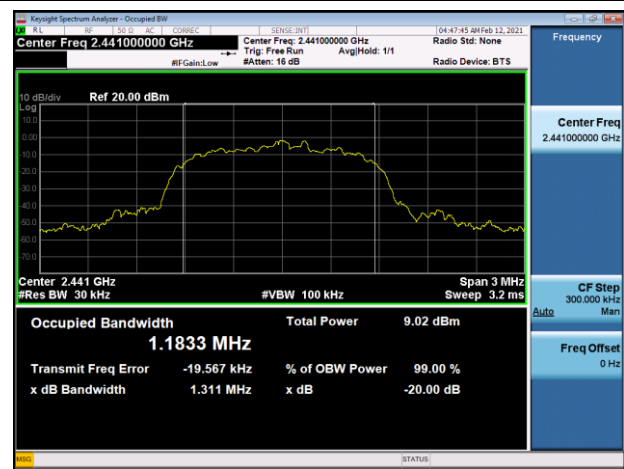
EDR (8DPSK) : 20dB BW / OBW (CH39)
