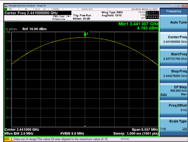
EDR (8DPSK) : Output Power (CH39)
