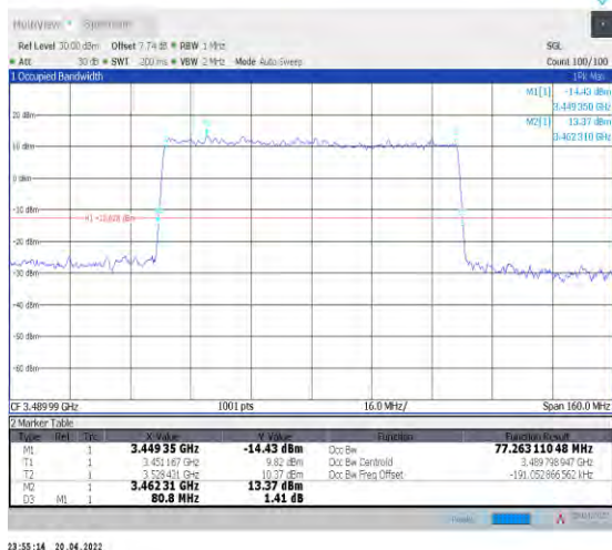
1-N78-3450-3550--30-80-L-5-DFT-256QAM-Outer_Full-216@0-Ant0-77.263-80.800-≤80-PASS
