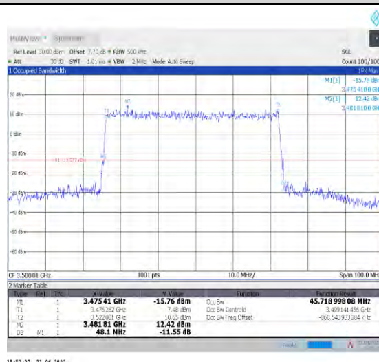
1-N78-3450-3550--30-50-M-4-DFT-64QAM-Outer_Full -128@0-Ant0-45.719-48.100-≤50-PASS
