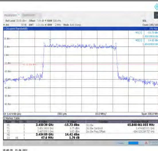
1-N78-3450-3550--30-50-L-1-DFT-QPSK-Outer_Full- 128@0-Ant0-45.848-47.600-≤50-PASS
