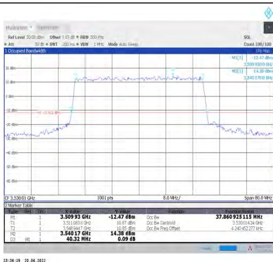
1-N78-3450-3550--30-40-H-7-CP-16QAM-Outer_Full -106@0-Ant0-37.861-40.320-≤40-PASS
