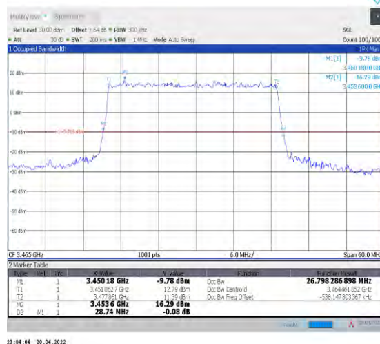
1-N78-3450-3550--30-30-L-1-DFT-QPSK-Outer_Full-75@0-Ant0-26.798-28.740-≤30-PASS
