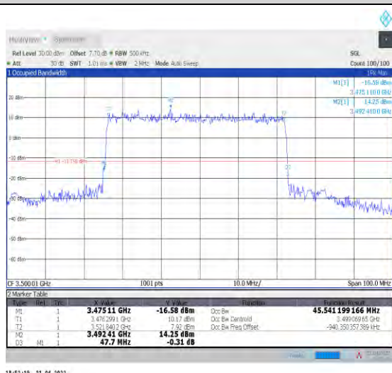
1-N78-3450-3550--30-50-M-3-DFT-16QAM-Outer_Full -128@0-Ant0-45.541-47.700-≤50-PASS
