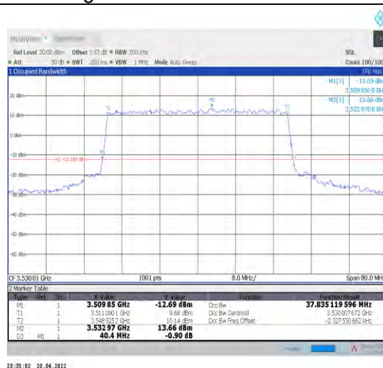
1-N78-3450-3550--30-40-H-8-CP-64QAM-Outer_Full -106@0-Ant0-37.835-40.400-≤40-PASS
