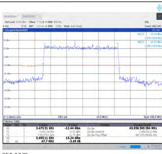
1-N78-3450-3550--30-50-M-1-DFT-QPSK-Outer_Full -128@0-Ant0-45.936-47.700-≤50-PASS
