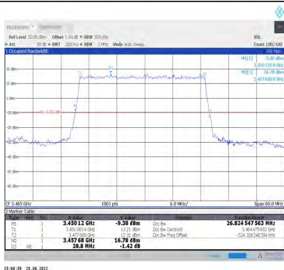
1-N78-3450-3550--30-30-L-2-DFT-PI2BPSK-Outer_Full-75@0-Ant0-26.825-28.800-≤30-PASS
