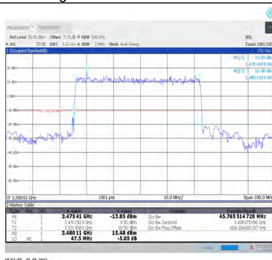
1-N78-3450-3550--30-50-M-2-DFT-PI2BPSK-Outer_Full -128@0-Ant0-45.766-47.500-≤50-PASS
