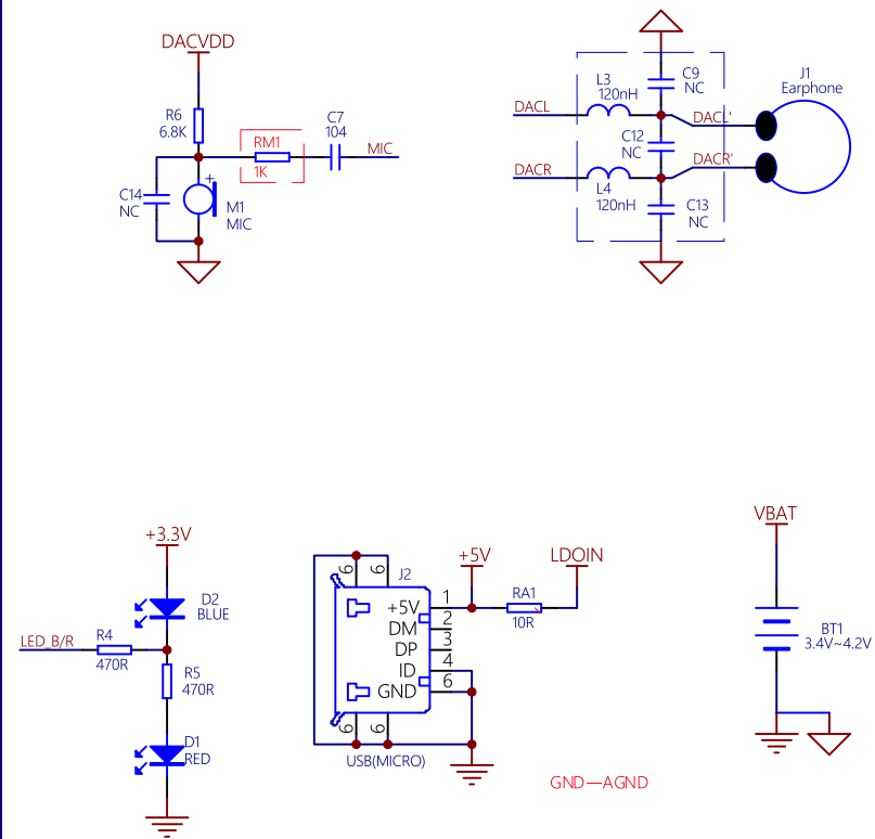
MIC —Earphone—LED —Power
