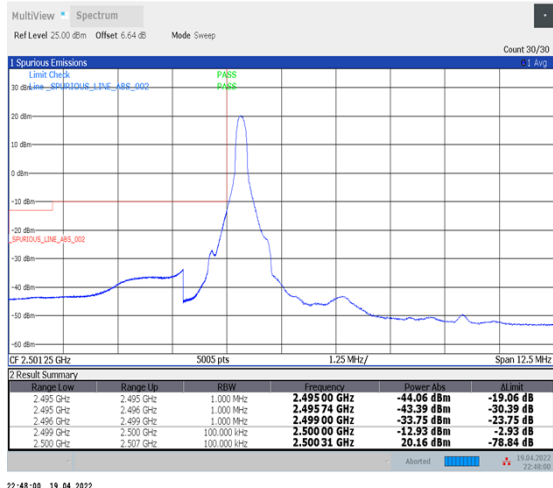
1-N7--15-5-L-1-DFT-PI2BPSK-Edge_1RB_Left-1@0-Ant1-PASS-see graph
