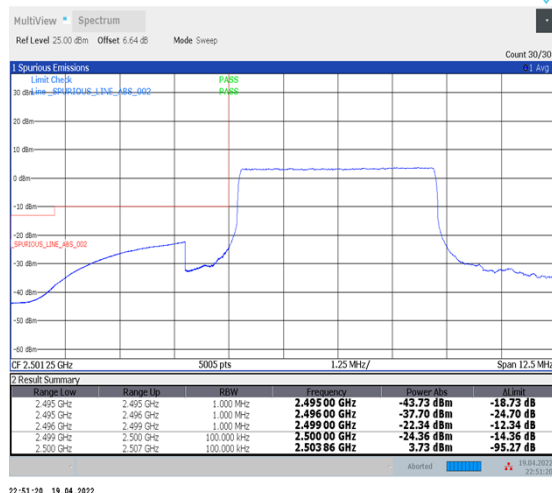
1-N7--15-5-L-6-CP-QPSK-Outer_Full-25@0-Ant1-PASS-see graph
