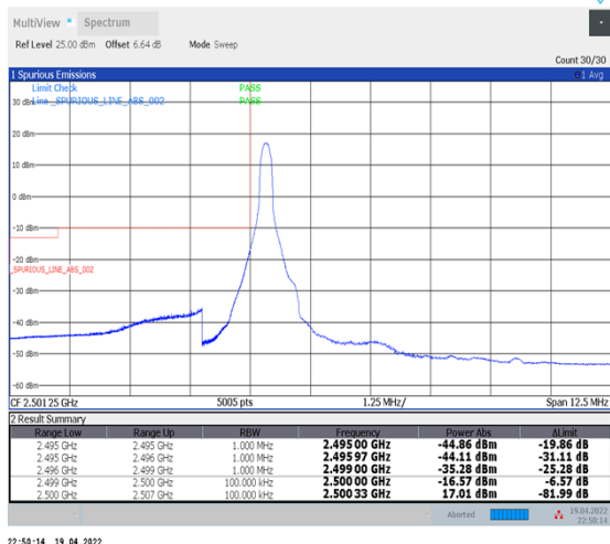
1-N7--15-5-L-4-CP-QPSK-Edge_1RB_Left-1@0-Ant1-PASS-see graph
