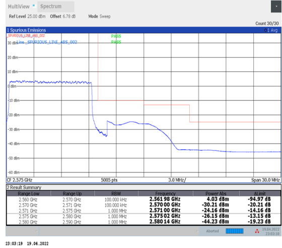
1-N7--15-10-H-3-DFT-PI2BPSK-Outer_Full-50@0-Ant1-PASS-see graph
