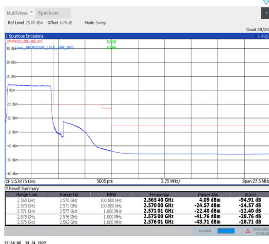
1-N7--15-5-H-6-CP-QPSK-Outer_Full-25@0-Ant1-PASS-see graph
