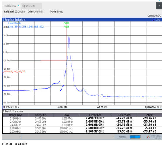
1-N7--15-10-L-1-DFT-PI2BPSK-Edge_1RB_Left-1@0-Ant1-PASS-see graph
