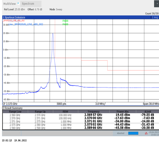
1-N7--15-10-H-2-DFT-PI2BPSK-Edge_1RB_Right-1@51-Ant1-PASS-see graph
