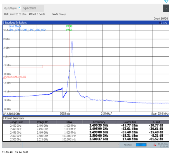
1-N7--15-10-L-4-CP-QPSK-Edge_1RB_Left-1@0-Ant1-PASS-see graph
