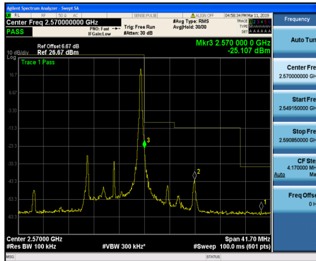
Band7_10MHz_QPSK_21400_1RB#49
