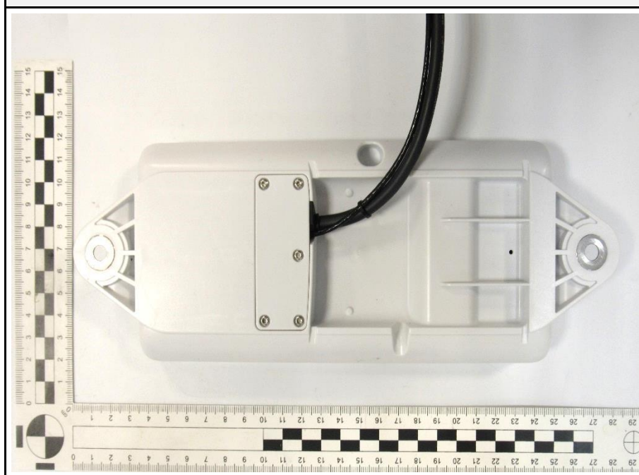
EUT 1 Bottom view 2
