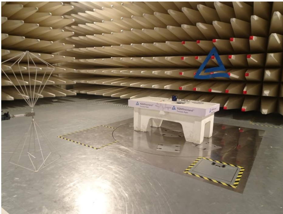
Test setup Frequency Range 30MHz-200MHz Biconical Antenna
