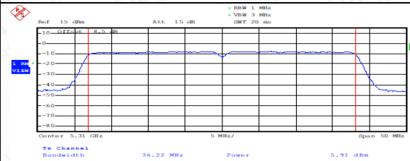
Output Power-Conducted (802.11n-HT40, Ch62)
