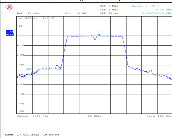
Power Spectral Density(dBm/MHz) (802.11n-HT40), 5230MHz)
