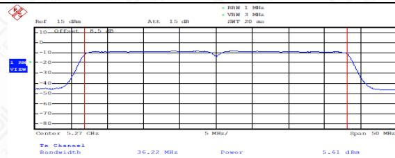
Output Power-Conducted (802.11n-HT40, Ch54)
