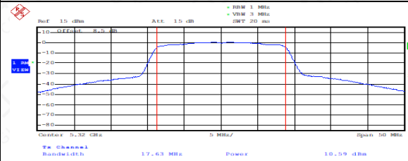
Output Power-Conducted (802.11n-HT20, Ch64)
