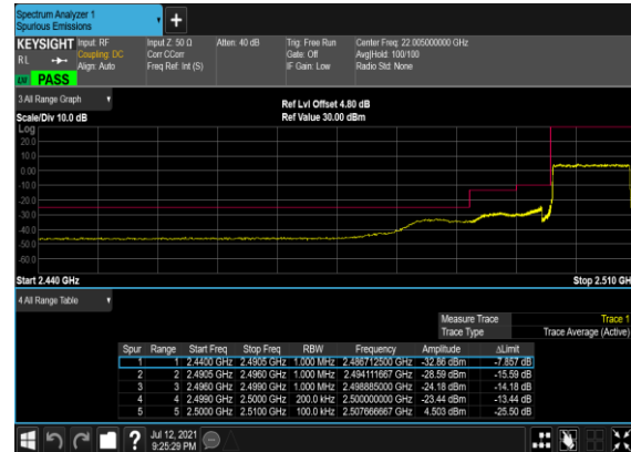
N7(10M)_DFT-s- OFDM_QPSK_Outer_Full_Low_CH
