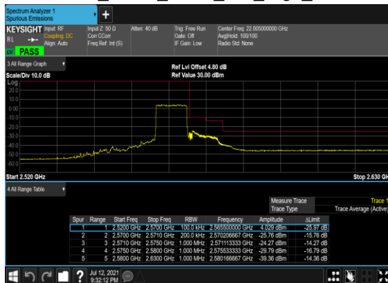
N7(10M)_DFT-s- OFDM_BPSK_Outer_Full_High_CH
