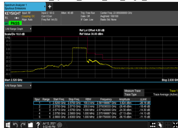
N7(10M)_DFT-s- OFDM_QPSK_Outer_Full_High_CH
