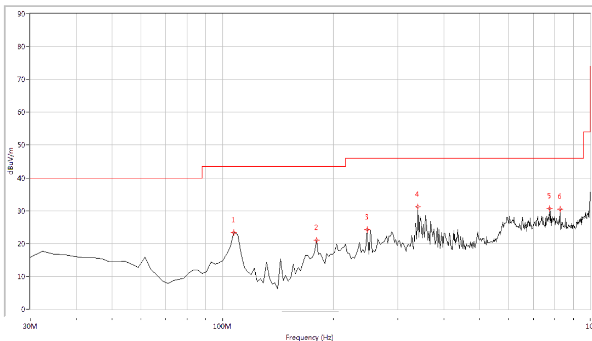
(Plot B: 30MHz – 1GHz, Test Antenna Horizontal)
