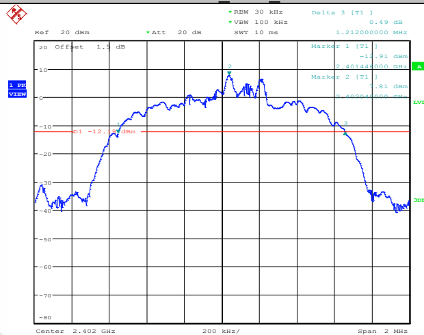
3DH5_Ant1_2402
