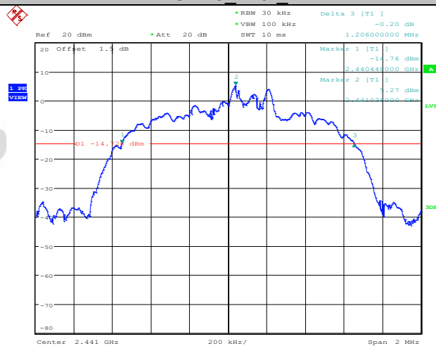
3DH5_Ant1_2441
