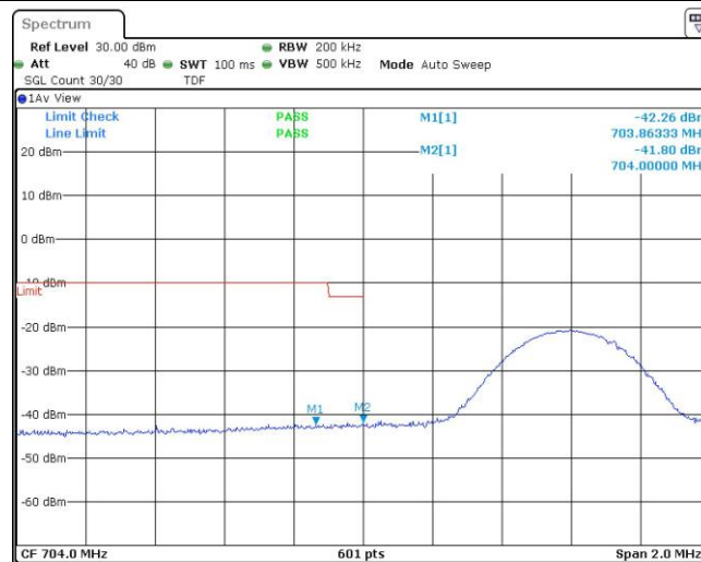
Band17-10MHz-QPSK-23780-50RB#0
