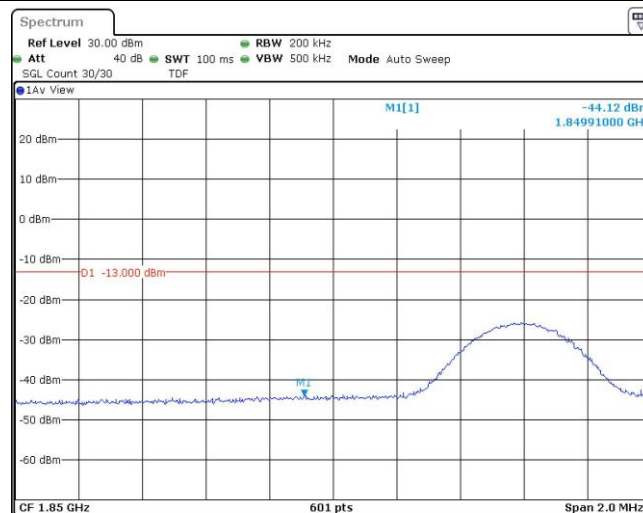
Band25-10MHz-QPSK-26090-50RB#0
