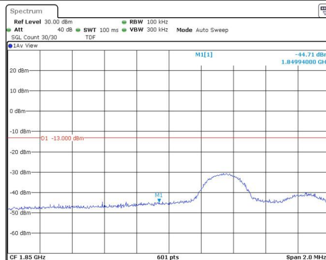
Band25-5MHz-QPSK-26065-25RB#0
