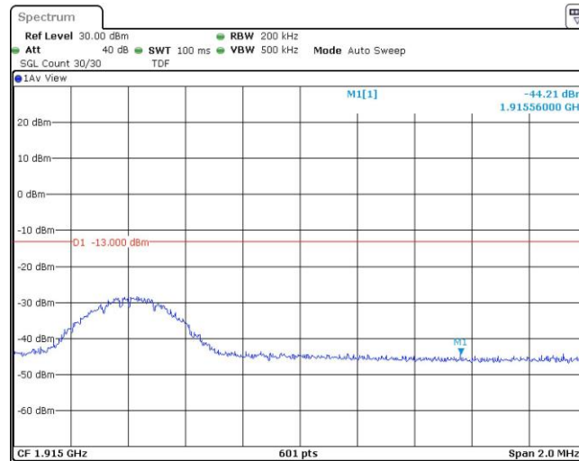
Band25-10MHz-16QAM-26640-1RB#49
