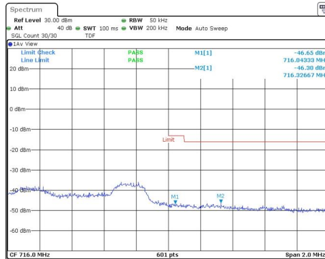
Band12-3MHz-16QAM-23165-1RB#14
