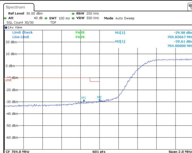
Band17-10MHz-16QAM-23800-1RB#0
