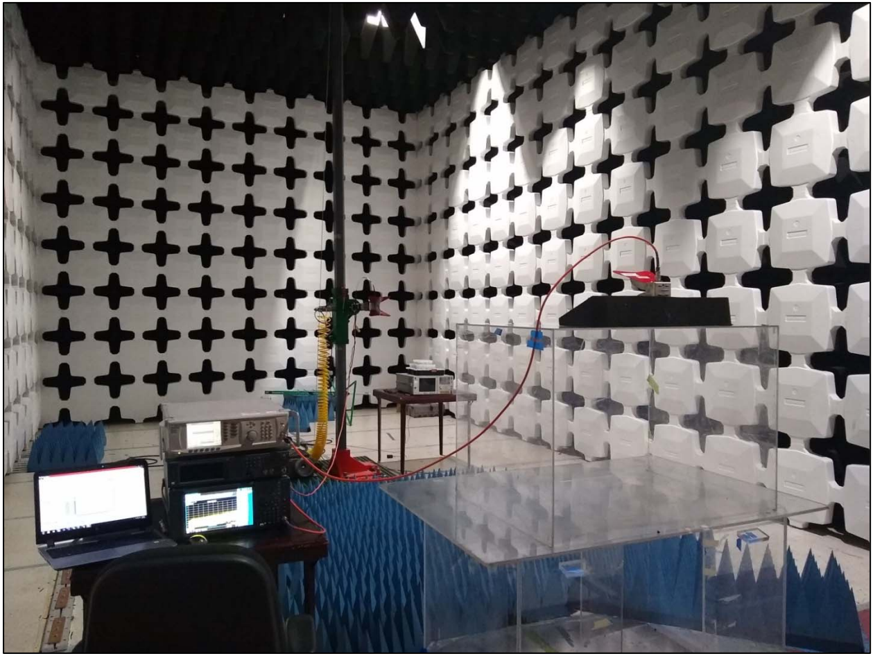
Substitution Method, Test Setup
