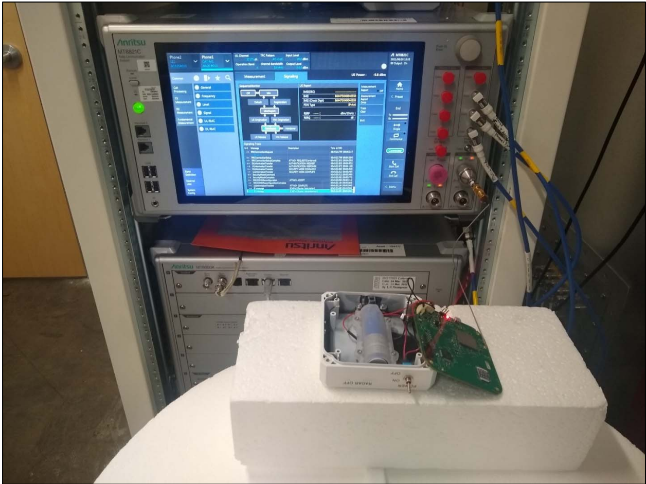
Conducted Power Measurement Test Setup
