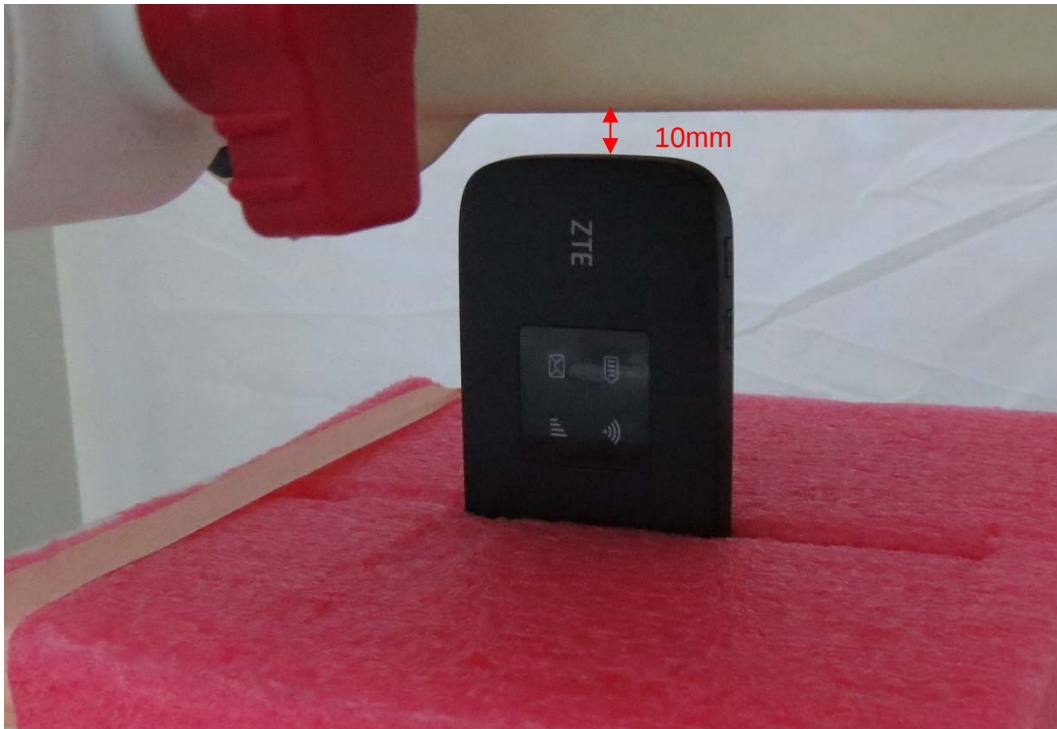
Picture 3: Left Side, the distance from handset to the bottom of the Phantom is 10mm
