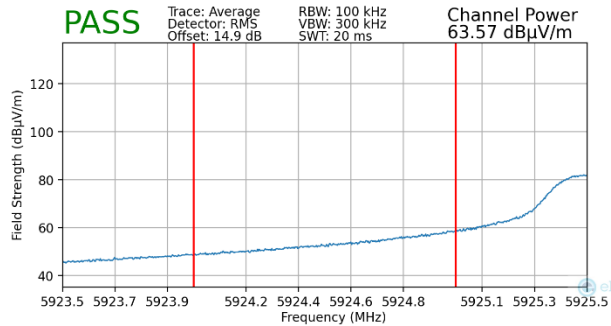
Plot 7-125. Radiated Lower Band Edge Plot MIMO (Average – UNII Band 5) with WCP
