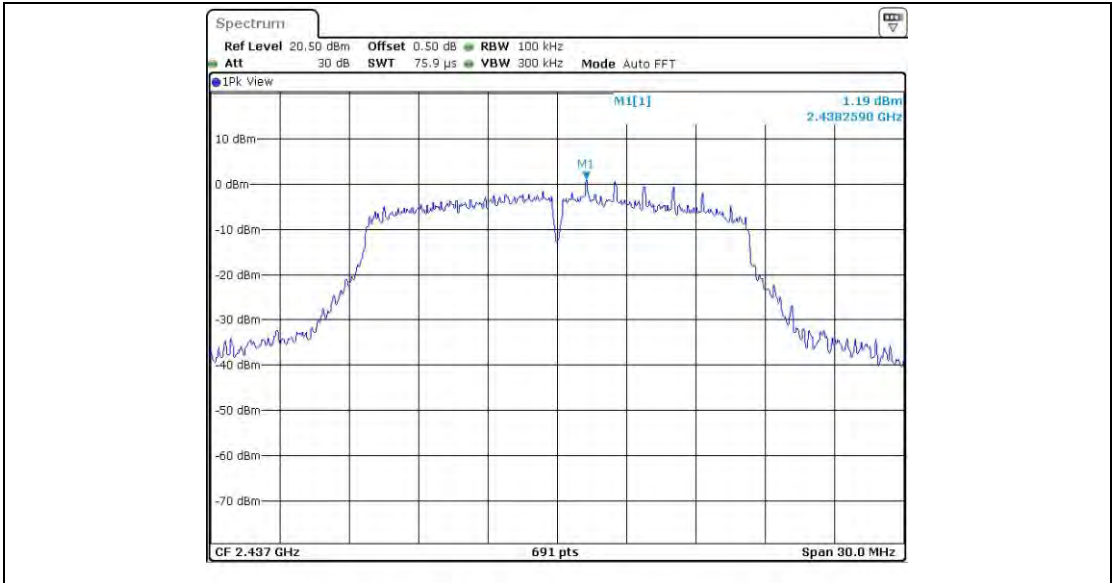
11G_Ant2_2437_0~Reference
