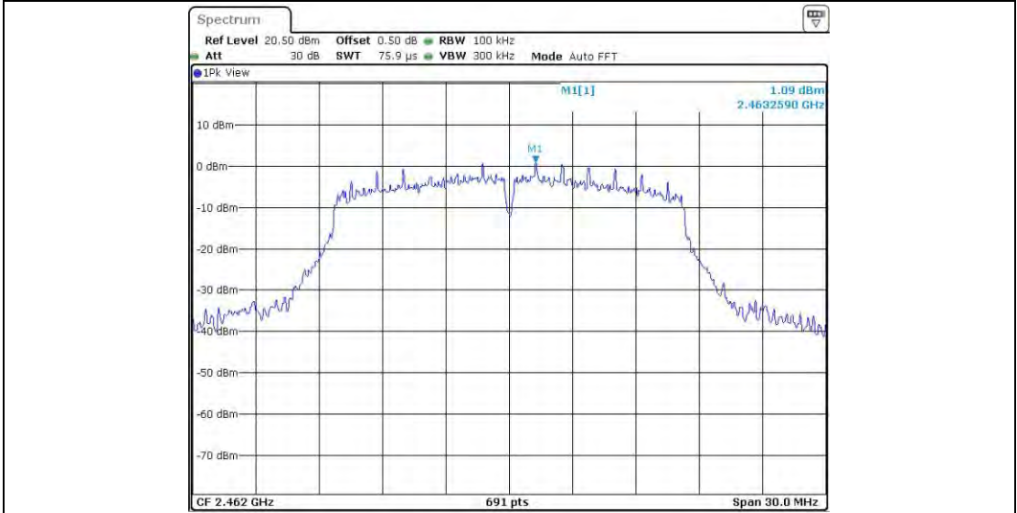
11G_Ant2_2462_0~Reference
