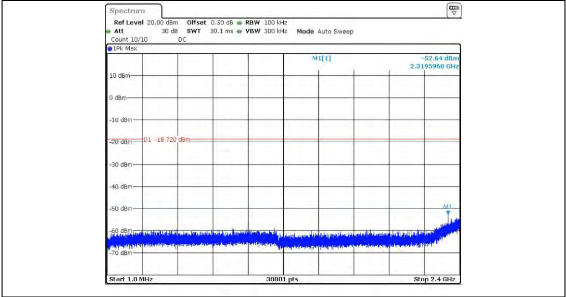
11N20_Ant1_2437_1~2400
