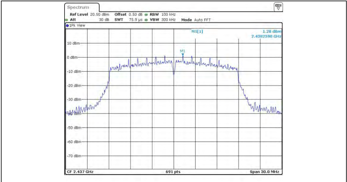
11N20_Ant1_2437_0~Reference
