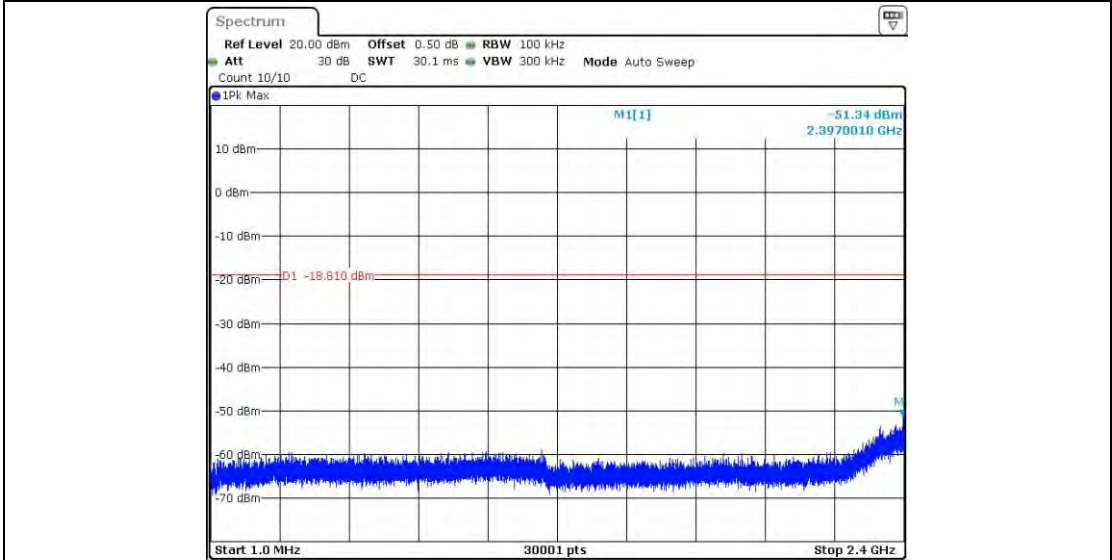
11G_Ant2_2437_0~Reference
