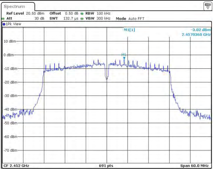
11N4OMIMO_Ant1_2452_0~Reference
