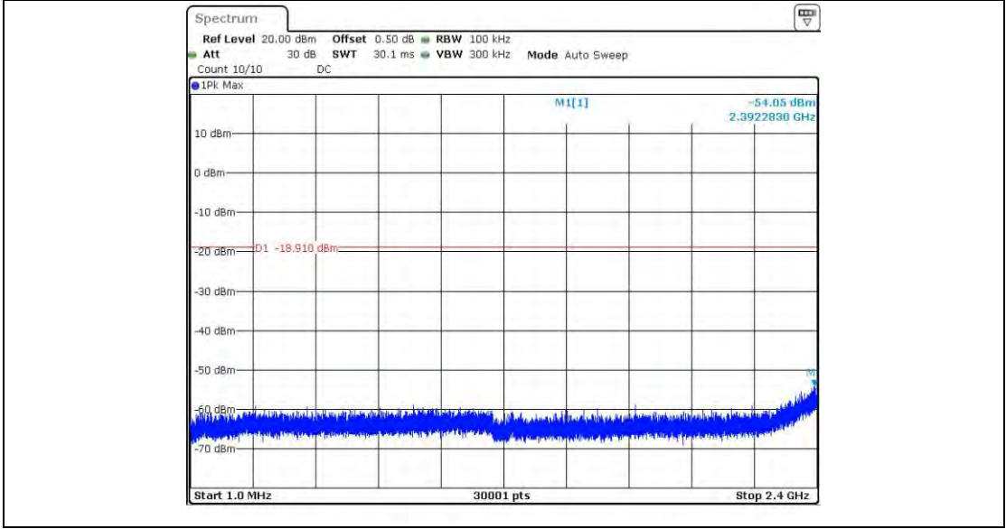
11G_Ant2_2462_0~Reference
