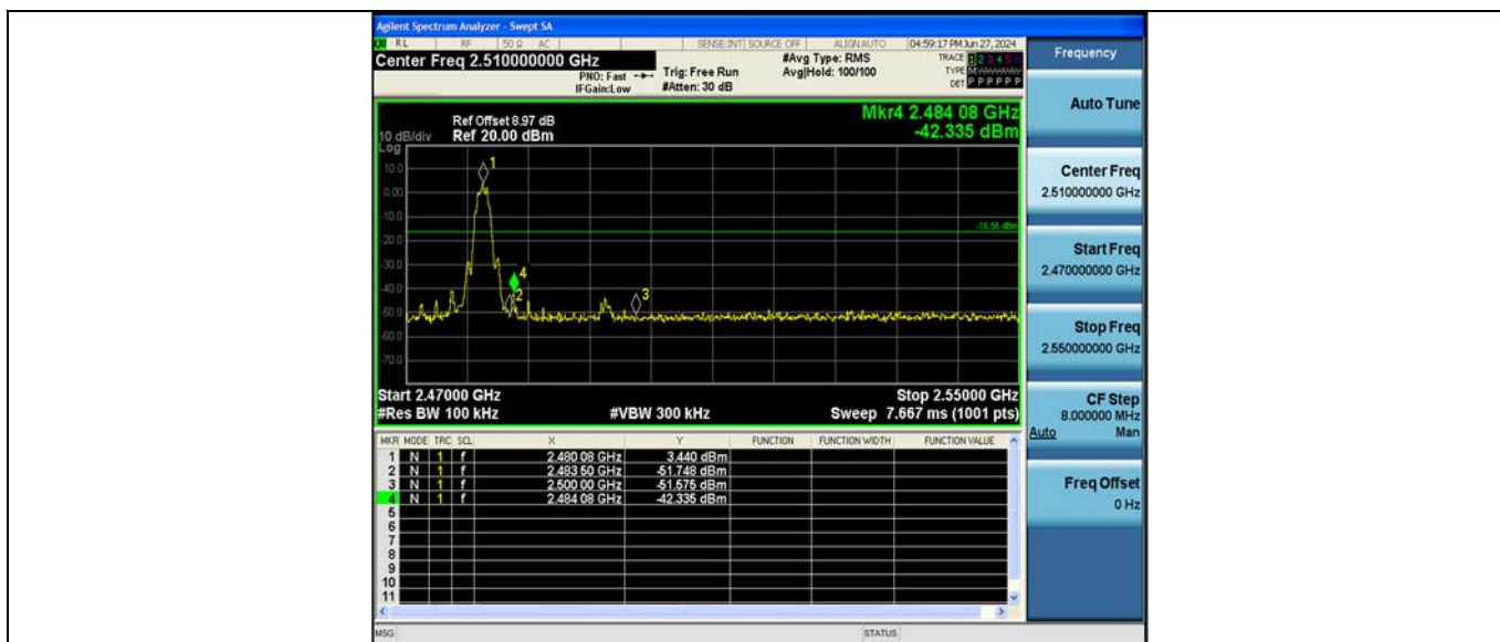
BLE_2M_Ant2_High_2480
