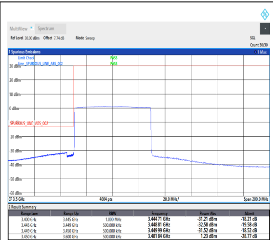
1-N78-3450-3550--30-60-L-6-CP-QPSK-Outer_Full-162@0-Ant1-1---see graph
