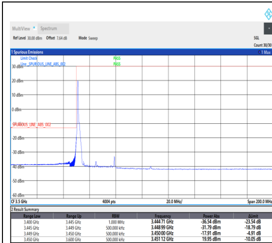
1-N78-3450-3550--30-30-L-4-CP-QPSK-Edge_1RB_Left-1@0-Ant1-1---see graph
