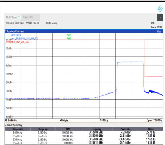
1-N78-3450-3550--30-30-H-6-CP-QPSK-Outer_Full-78@0-Ant1-1---see graph
