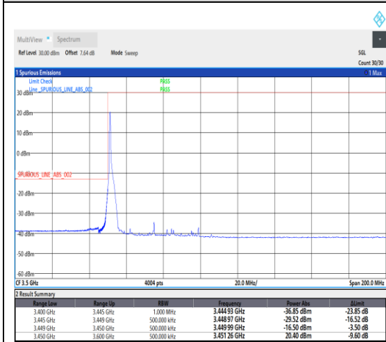
1-N78-3450-3550--30-50-L-1-DFT-PI2BPSK-Edge_1RB_Left-1@0-Ant1-1---see graph
