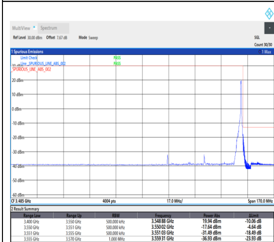
1-N78-3450-3550--30-50-H-5-CP-QPSK-Edge_1RB_Right-1@132-Ant1-1---see graph
