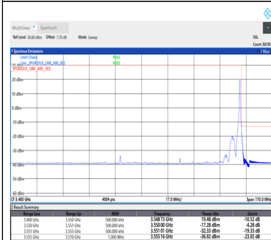
1-N78-3450-3550--30-80-H-2-DFT-PI2BPSK-Edge_1RB_Right-1@216-Ant1-1---see graph
