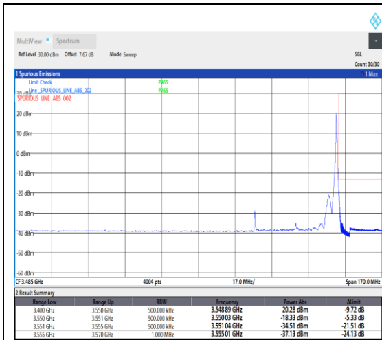
1-N78-3450-3550--30-40-H-5-CP-QPSK-Edge_1RB_Right-1@105-Ant1-1---see graph
