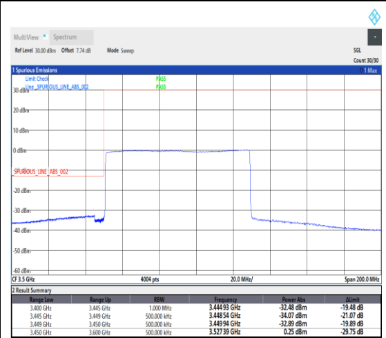
1-N78-3450-3550--30-80-L-6-CP-QPSK-Outer_Full-217@0-Ant1-1---see graph
