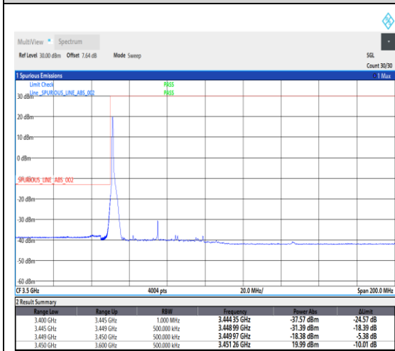
1-N78-3450-3550--30-50-L-4-CP-QPSK-Edge_1RB_Left-1@0-Ant1-1---see graph
