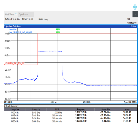
1-N78-3450-3550--30-40-L-3-DFT-PI2BPSK-Outer_Full-100@0-Ant1-1---see graph
