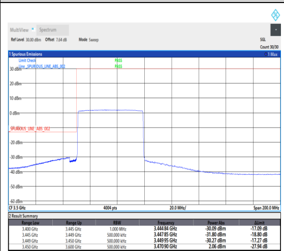
1-N78-3450-3550--30-50-L-6-CP-QPSK-Outer_Full-133@0-Ant1-1---see graph
