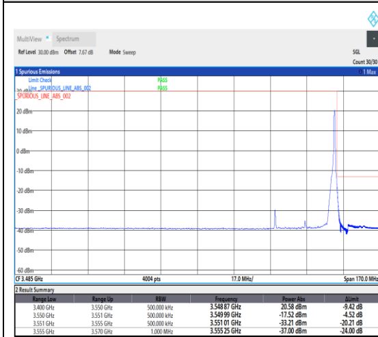
1-N78-3450-3550--30-30-H-2-DFT-PI2BPSK-Edge_1RB_Right-1@77-Ant1-1---see graph
