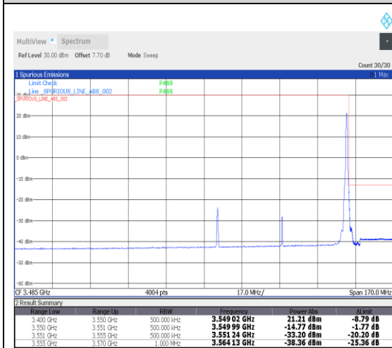
1-N78-3450-3550--30-60-H-5-CP-QPSK-Edge_1RB_Right-1@161-Ant1-1---see graph
