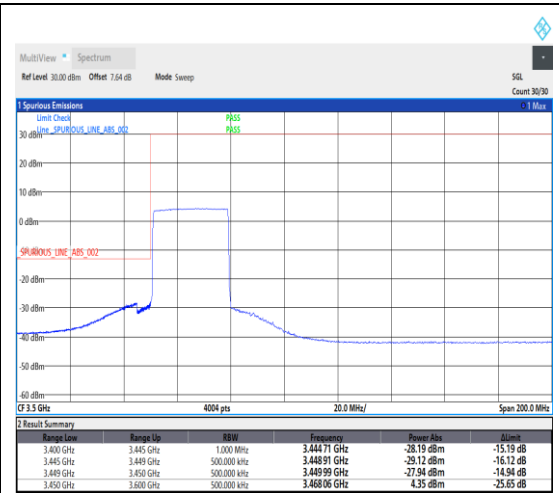
1-N78-3450-3550--30-30-L-6-CP-QPSK-Outer_Full-78@0-Ant1-1---see graph
