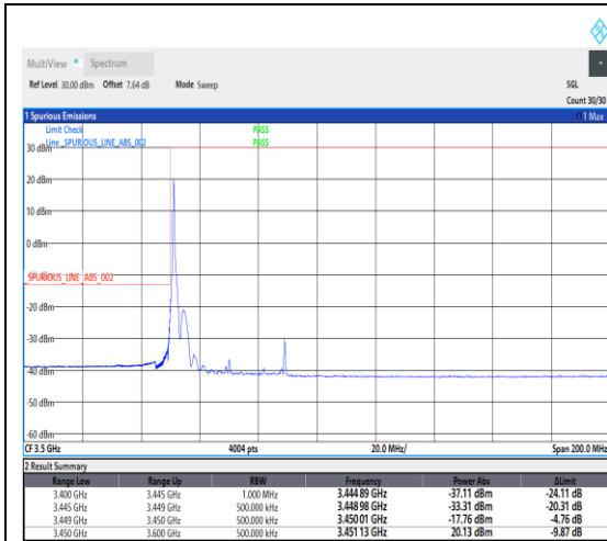
1-N78-3450-3550--30-40-L-1-DFT-PI2BPSK-Edge_1RB_Left-1@0-Ant1-1---see graph
