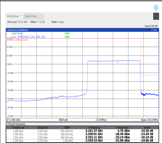
1-N78-3450-3550--30-60-H-3-DFT-PI2BPSK-Outer_Full-162@0-Ant1-1---see graph
