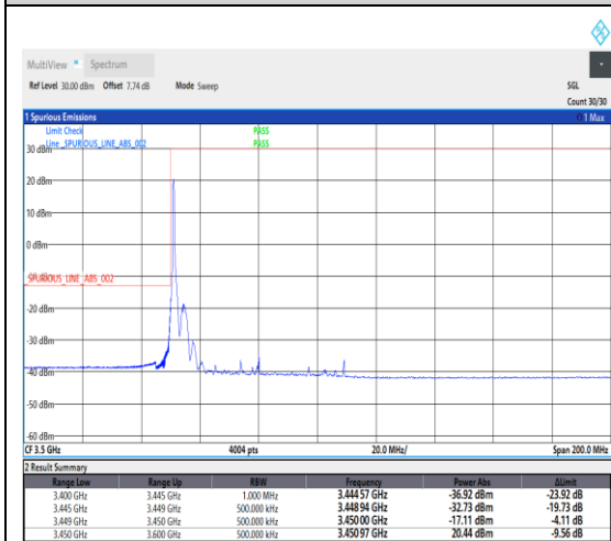
1-N78-3450-3550--30-60-L-1-DFT-PI2BPSK-Edge_1RB_Left-1@0-Ant1-1---see graph
