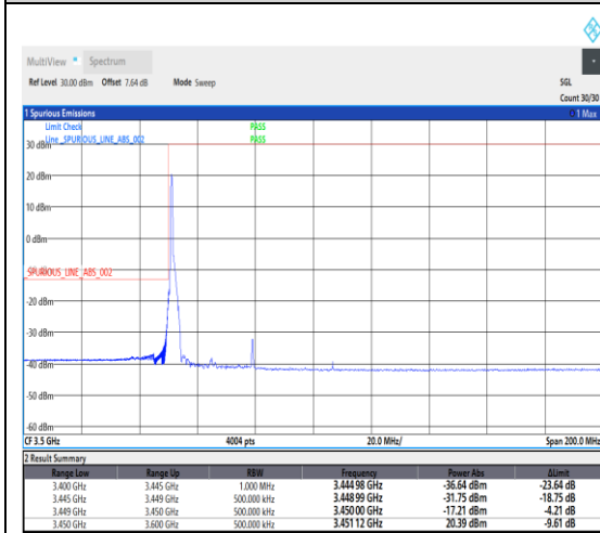
1-N78-3450-3550--30-30-L-1-DFT-PI2BPSK-Edge_1RB_Left-1@0-Ant1-1---see graph
