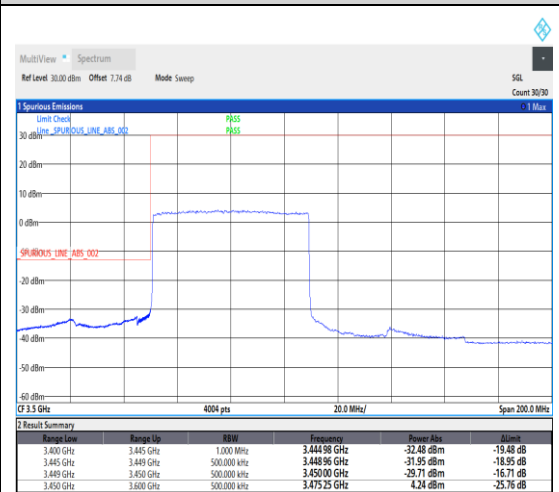
1-N78-3450-3550--30-60-L-3-DFT-PI2BPSK-Outer_Full-162@0-Ant1-1---see graph
