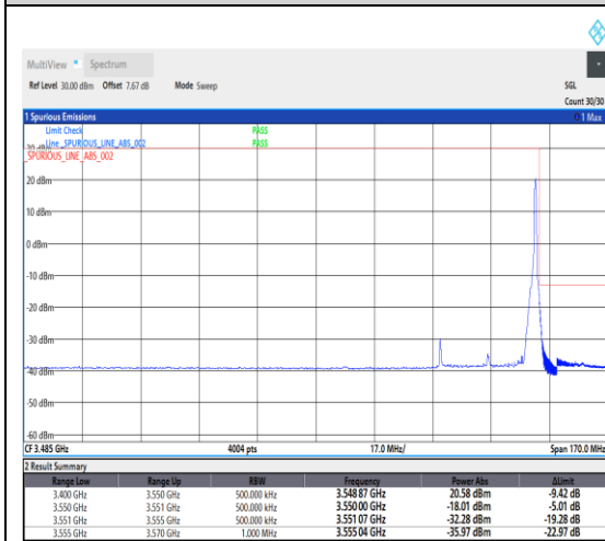
1-N78-3450-3550--30-30-H-5-CP-QPSK-Edge_1RB_Right-1@77-Ant1-1---see graph
