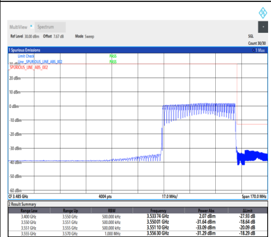
1-N78-3450-3550--30-50-H-6-CP-QPSK-Outer_Full-133@0-Ant1-1---see graph
