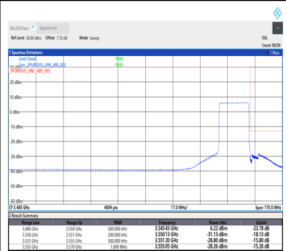
1-N78-3450-3550--30-20-H-6-CP-QPSK-Outer_Full-51@0-Ant1-1---see graph
