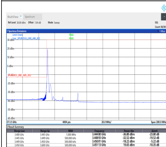
1-N78-3450-3550--30-40-L-4-CP-QPSK-Edge_1RB_Left-1@0-Ant1-1---see graph
