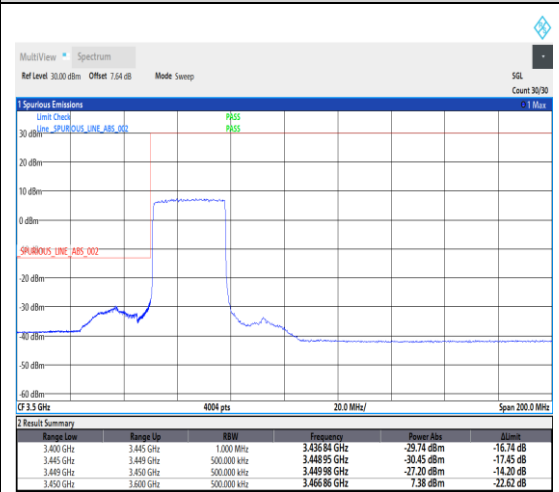
1-N78-3450-3550--30-30-L-3-DFT-PI2BPSK-Outer_Full-75@0-Ant1-1---see graph
