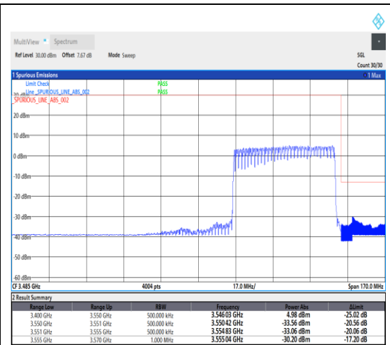
1-N78-3450-3550--30-50-H-3-DFT-PI2BPSK-Outer_Full-128@0-Ant1-1---see graph
