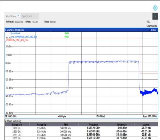
1-N78-3450-3550--30-80-H-3-DFT-PI2BPSK-Outer_Full-216@0-Ant1-1---see graph
