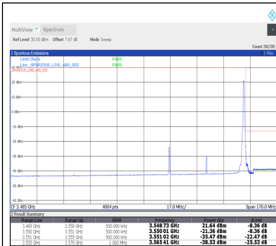
1-N78-3450-3550--30-50-H-2-DFT-PI2BPSK-Edge_1RB_Right-1@132-Ant1-1---see graph
