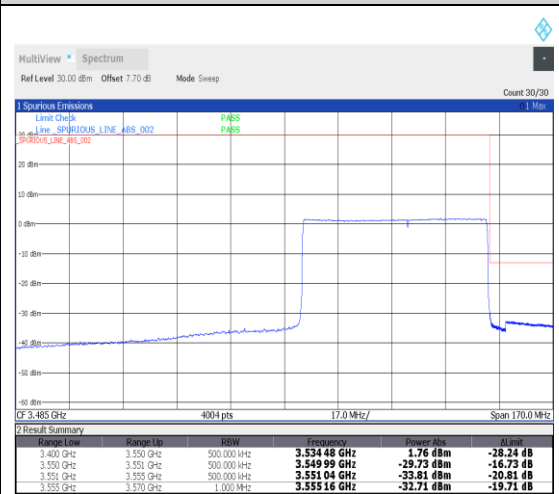
1-N78-3450-3550--30-60-H-6-CP-QPSK-Outer_Full-162@0-Ant1-1---see graph
