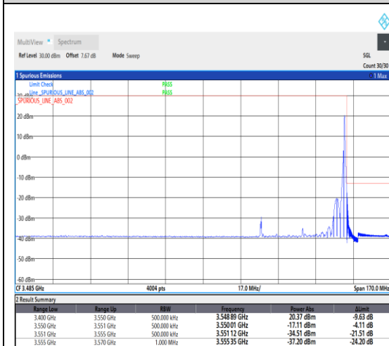
1-N78-3450-3550--30-40-H-2-DFT-PI2BPSK-Edge_1RB_Right-1@105-Ant1-1---see graph
