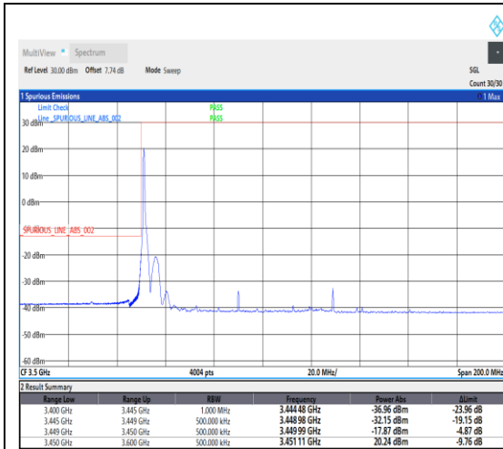
1-N78-3450-3550--30-80-L-1-DFT-PI2BPSK-Edge_1RB_Left-1@0-Ant1-1---see graph
