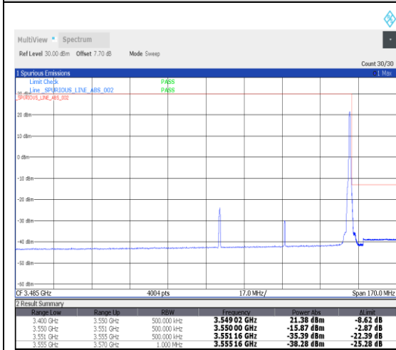
1-N78-3450-3550--30-60-H-2-DFT-PI2BPSK-Edge_1RB_Right-1@161-Ant1-1---see graph
