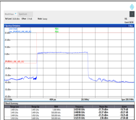
1-N78-3450-3550--30-80-L-3-DFT-PI2BPSK-Outer_Full-216@0-Ant1-1---see graph
