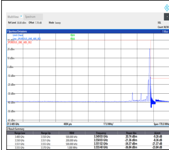
1-N78-3450-3550--30-20-H-5-CP-QPSK-Edge_1RB_Right-1@50-Ant1-1---see graph
