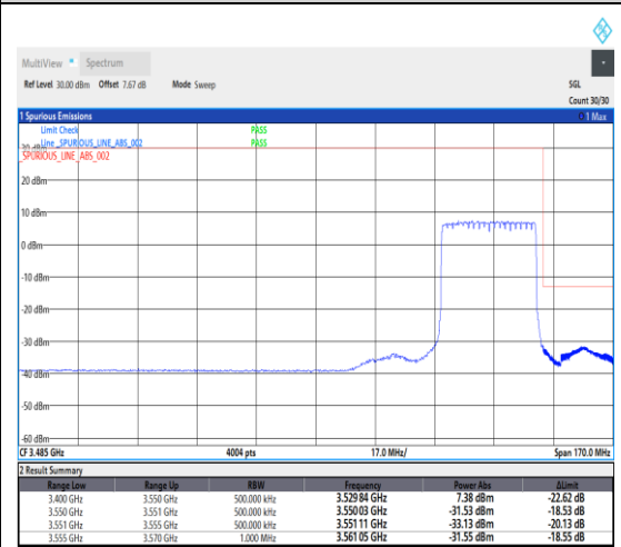
1-N78-3450-3550--30-30-H-3-DFT-PI2BPSK-Outer_Full-75@0-Ant1-1---see graph
