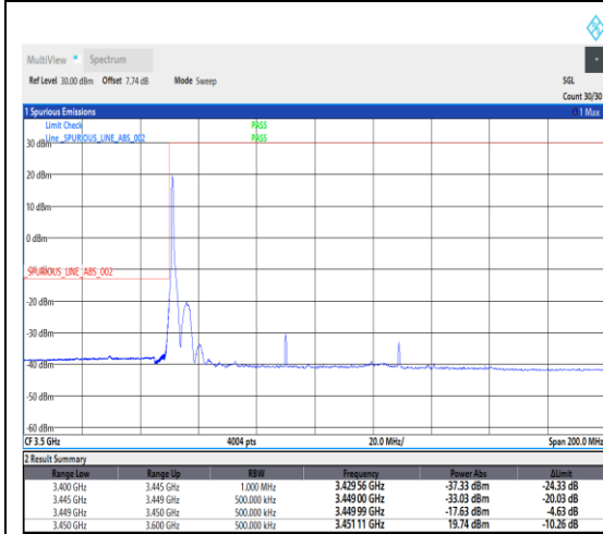
1-N78-3450-3550--30-80-L-4-CP-QPSK-Edge_1RB_Left-1@0-Ant1-1---see graph
