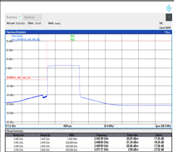
1-N78-3450-3550--30-40-L-6-CP-QPSK-Outer_Full-106@0-Ant1-1---see graph
