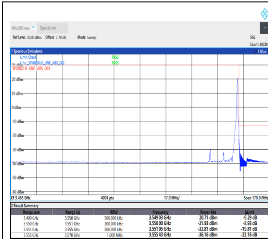
1-N78-3450-3550--30-20-H-2-DFT-PI2BPSK-Edge_1RB_Right-1@50-Ant1-1---see graph
