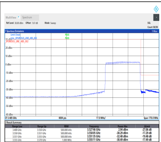
1-N78-3450-3550--30-40-H-6-CP-QPSK-Out_er_Full-106@0-Ant1-1---see graph
