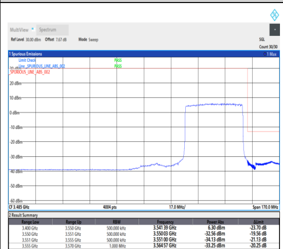
1-N78-3450-3550--30-40-H-3-DFT-PI2BPSK-Outer_Full-100@0-Ant1-1---see graph
