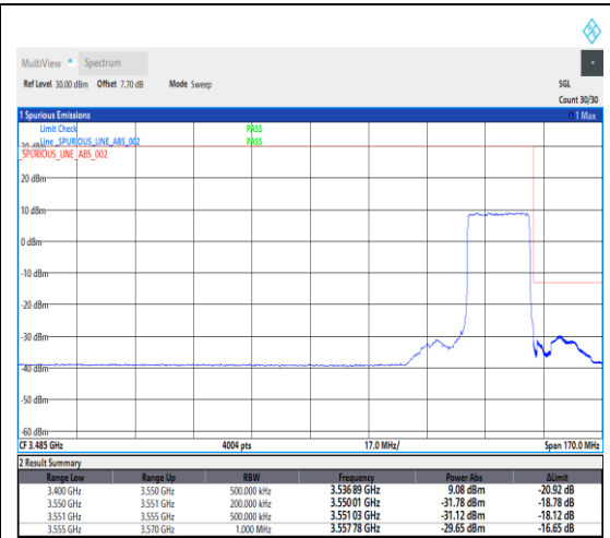
1-N78-3450-3550--30-20-H-3-DFT-PI2BPSK-Outer_Full-50@0-Ant1-1---see graph
