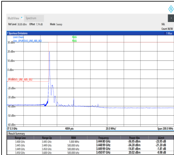
1-N78-3450-3550--30-60-L-4-CP-QPSK-Edge_1RB_Left-1@0-Ant1-1---see graph
