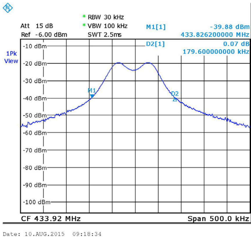
Figure 20. 433.92MHz
