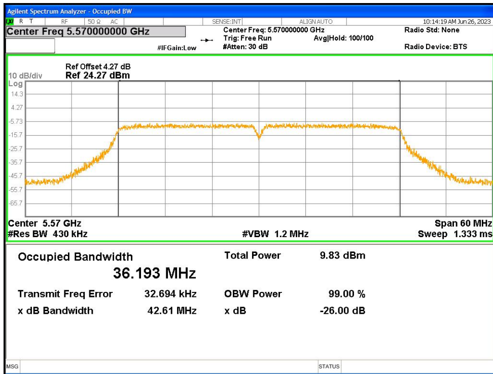
OBW NVNT ac40 5570MHz Ant2
