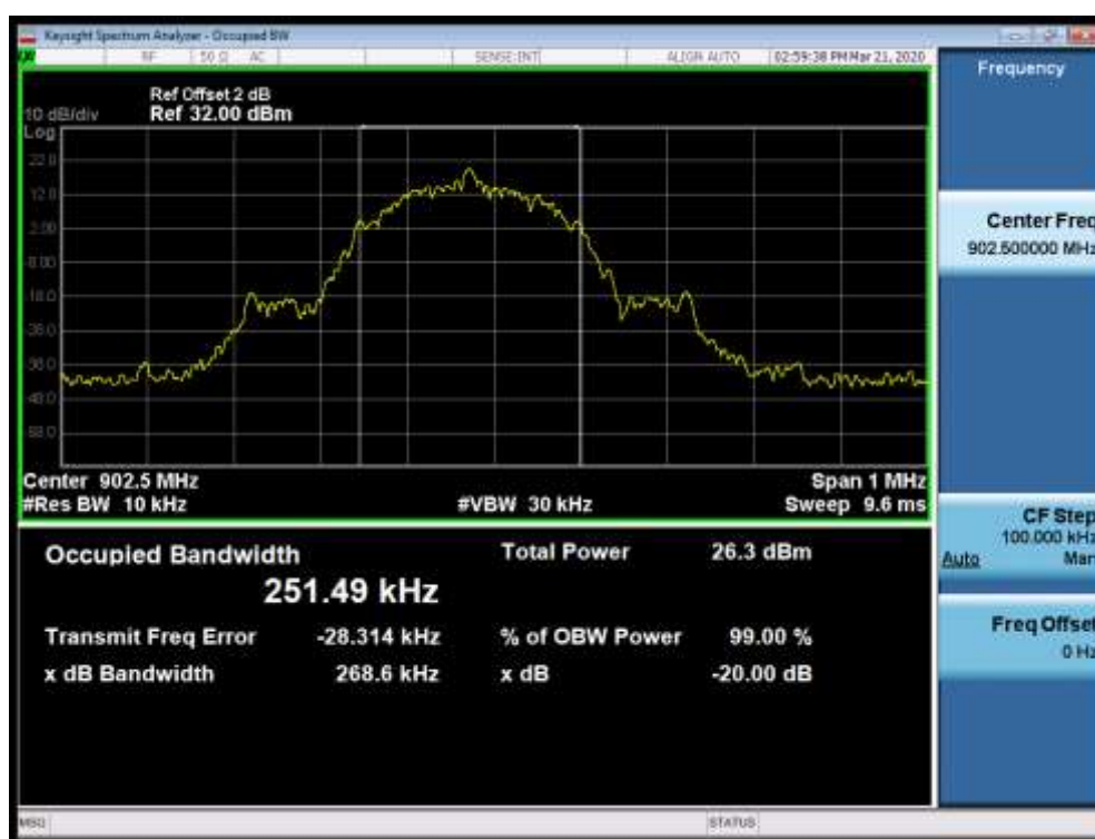
Channel 01 (902.5MHz)
