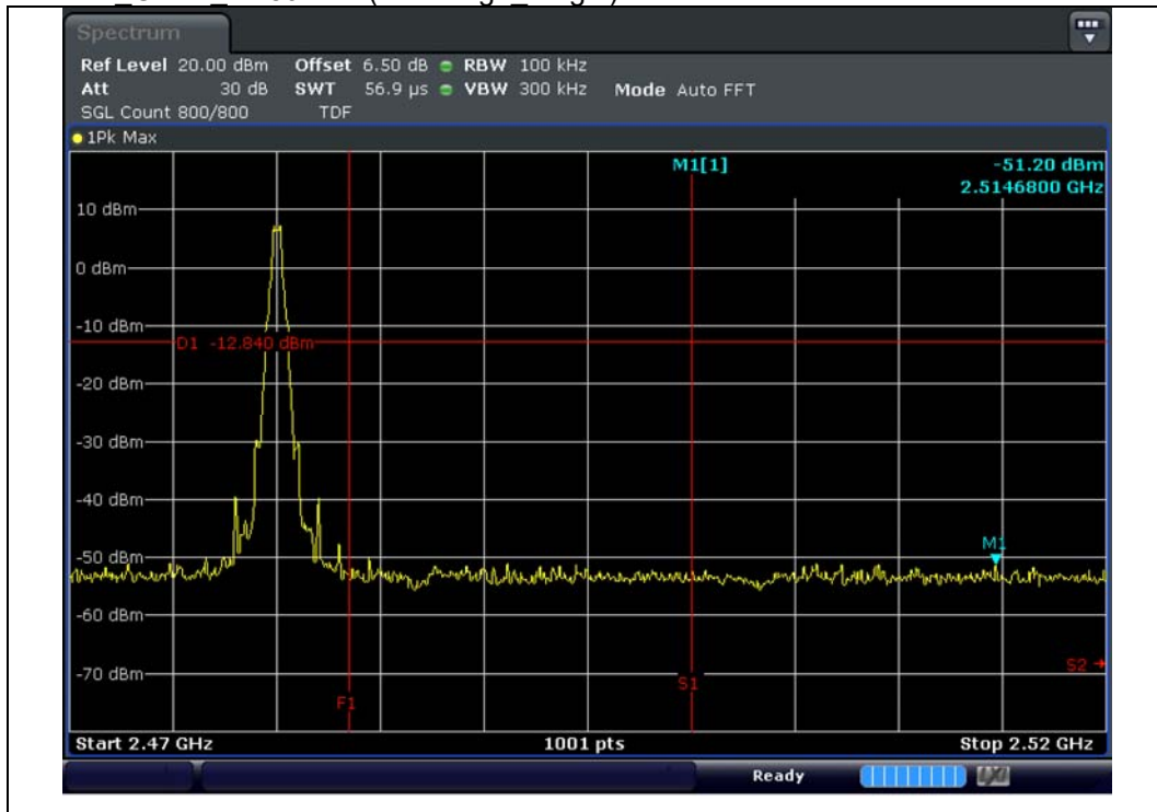
SLAVE_GFSK_2480 MHz(Bandedge Single)
