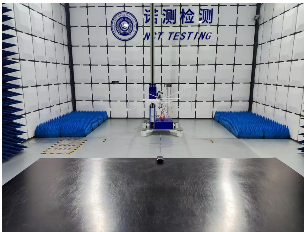
Setup Photo FCC ID: 2A90XB BP72141V
