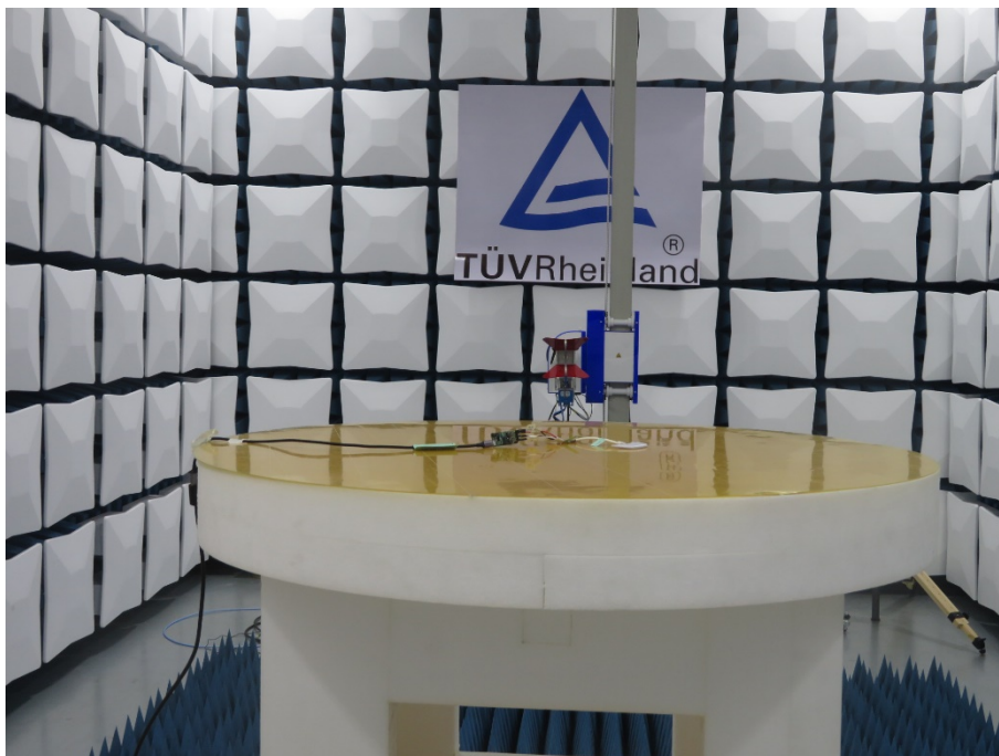
Photograph 6: Set-up for Radiated Spurious Emission, Above 1GHz
