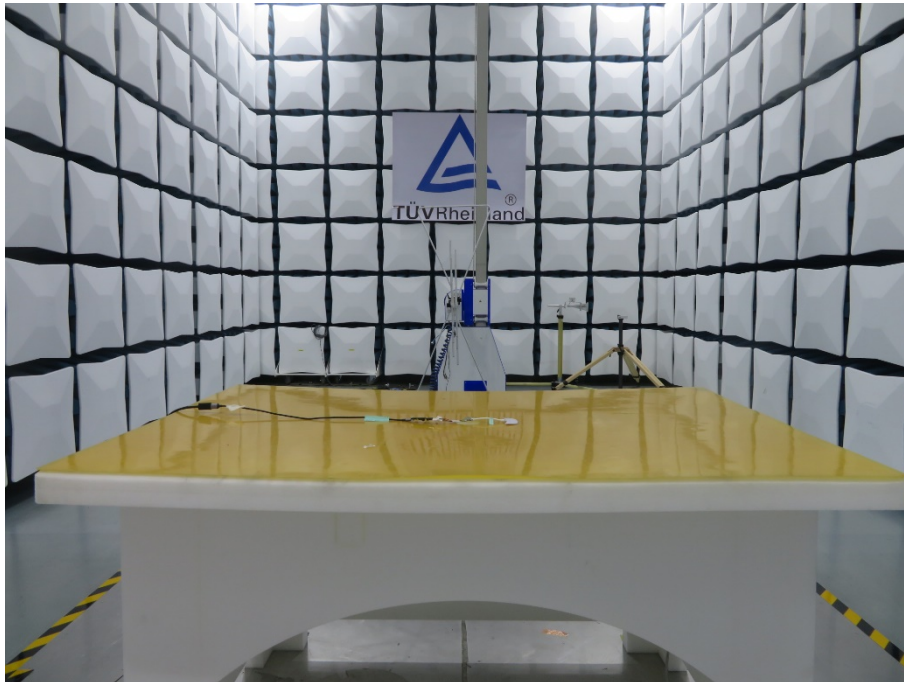
Photograph 5: Set-up for Radiated Spurious Emission, Below 1GHz
