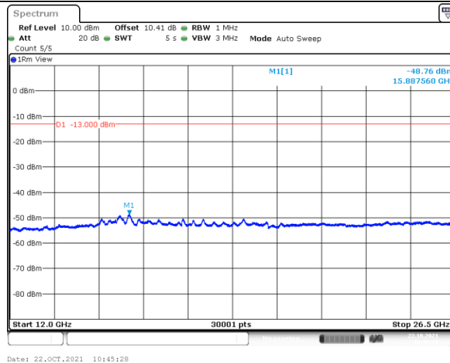
Band66-1.4MHz-16QAM-131979-1-0-Low-30-1000--34.71-PASS
