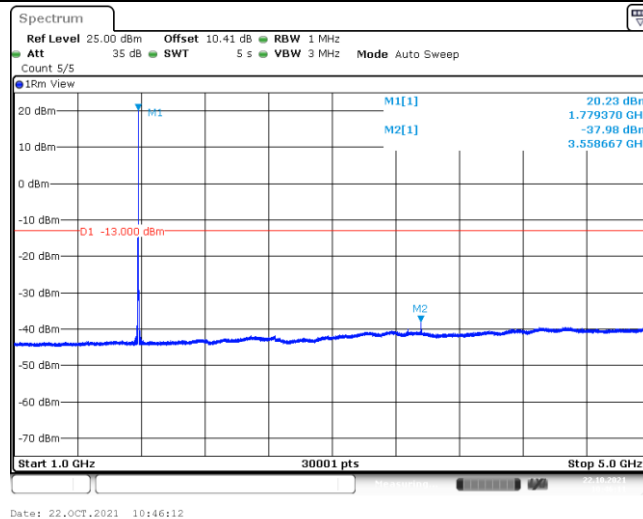
Band66-1.4MHz-16QAM-132665-6-0-Low-5000-12000--51.14-PASS
