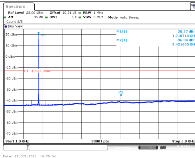
Band66-1.4MHz-QPSK-131979-6-0-Low-5000-12000--51.38-PASS
