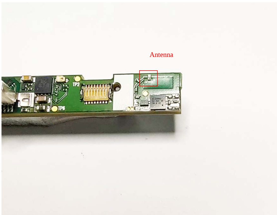
Inner Circuit Bottom View
