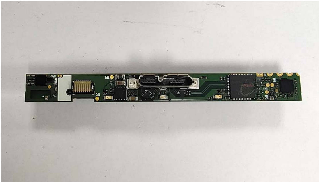
Inner Circuit Bottom View
