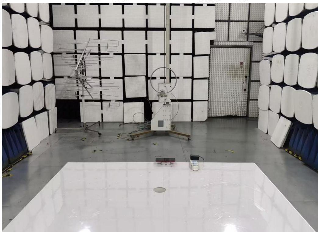
Radiated Emission below 30MHz-AC adapter charge mode
