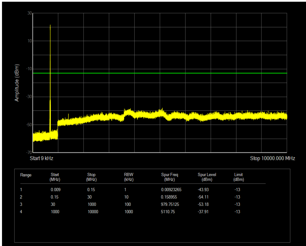
n12 SCS=30kHz DFT_QPSK BW=15MHz Channel=141300 RB=1@0
