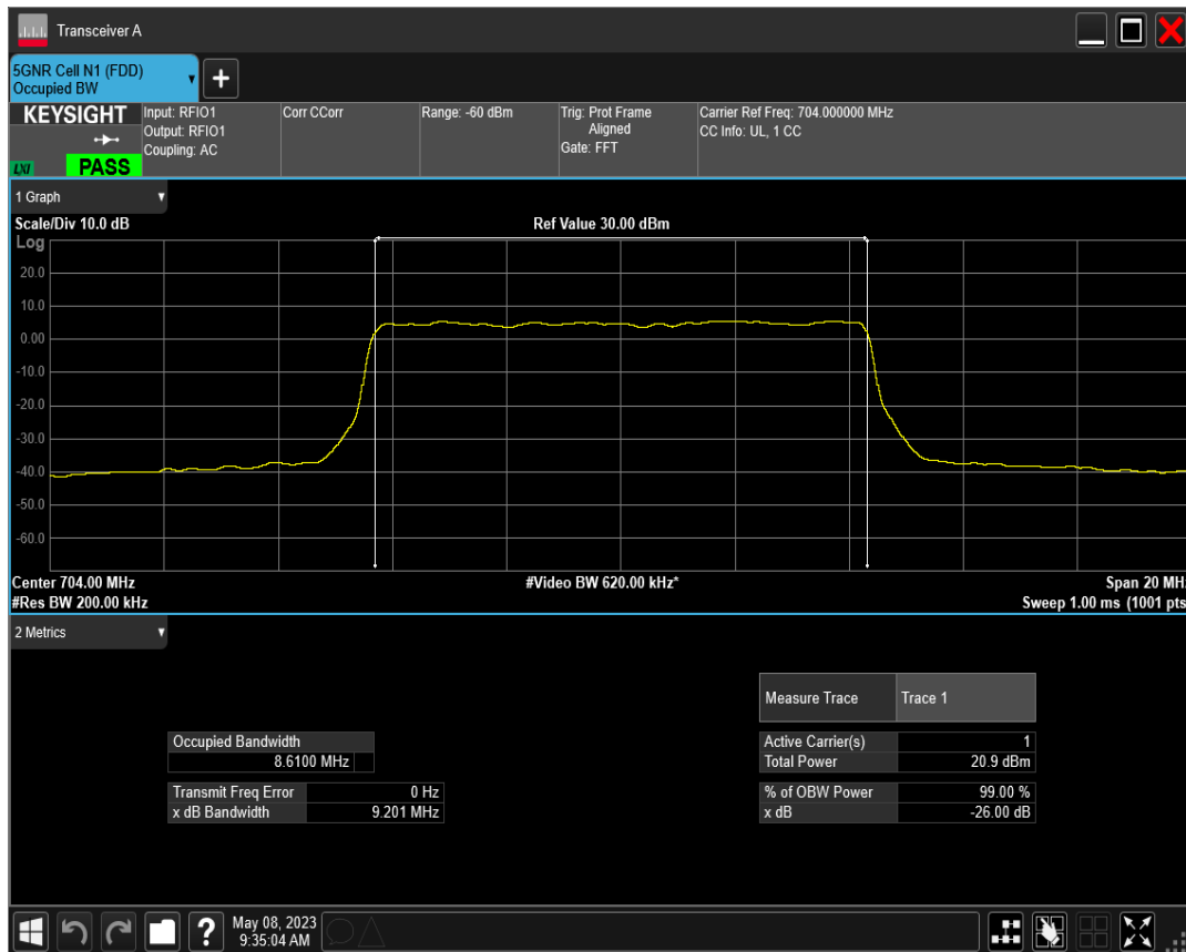
n12 SCS=30kHz DFT_QAM64 BW=10MHz Channel=140800 RB=24@0
