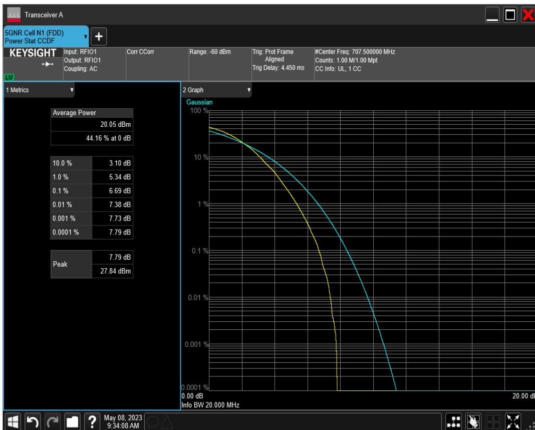
n12 SCS=30kHz DFT_QAM256 BW=15MHz Channel=141500 RB=36@0
