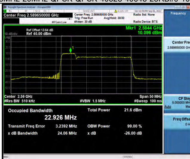
41C-5MHz-20MHz-QPSK-QPSK-41373-41490-25RB#0-100RB#0
