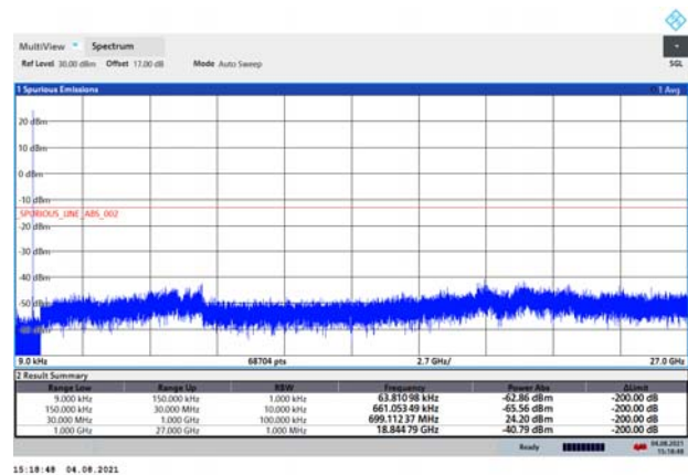
NB-IoT Band 12 CH-Middle 9kHz~27GHz
